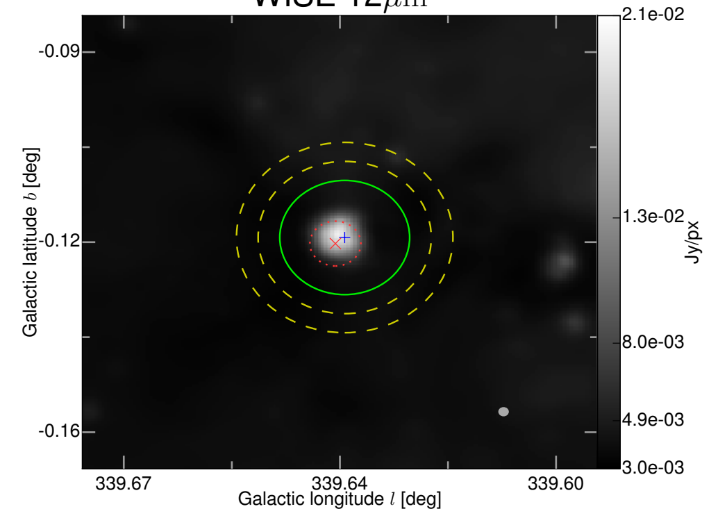
WISE 12\mu\text{m}
