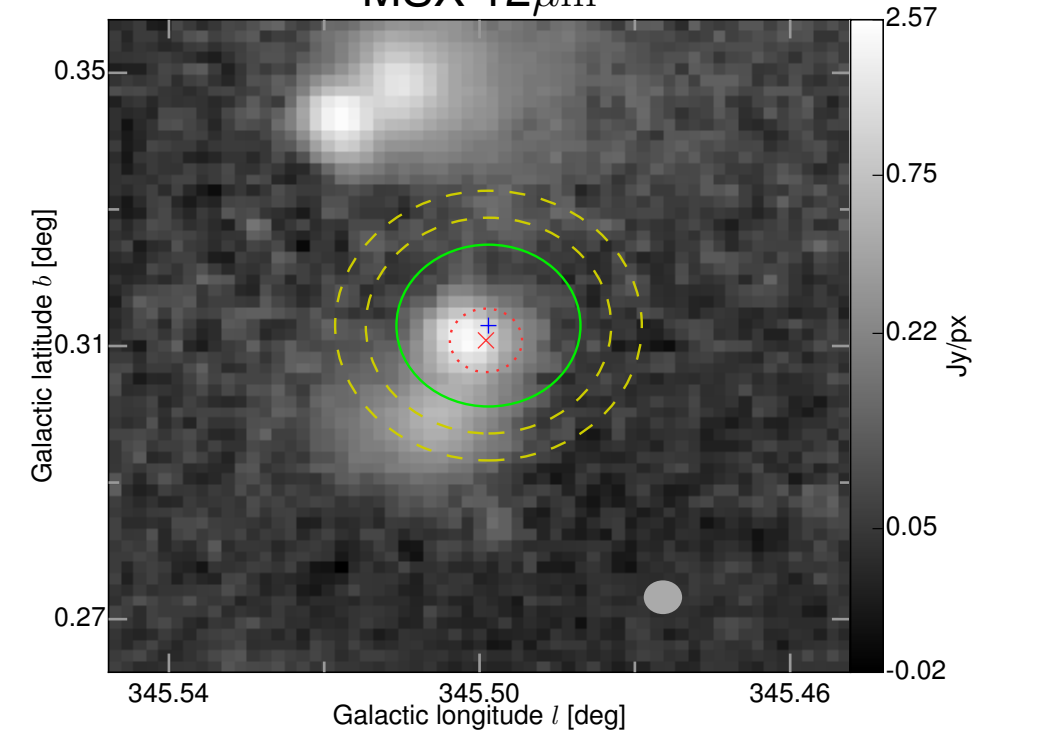
MSX 12 \mu\text{m}
