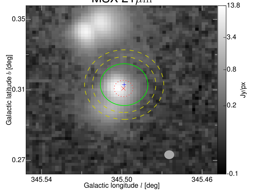
MSX 21 \mu\text{m}
