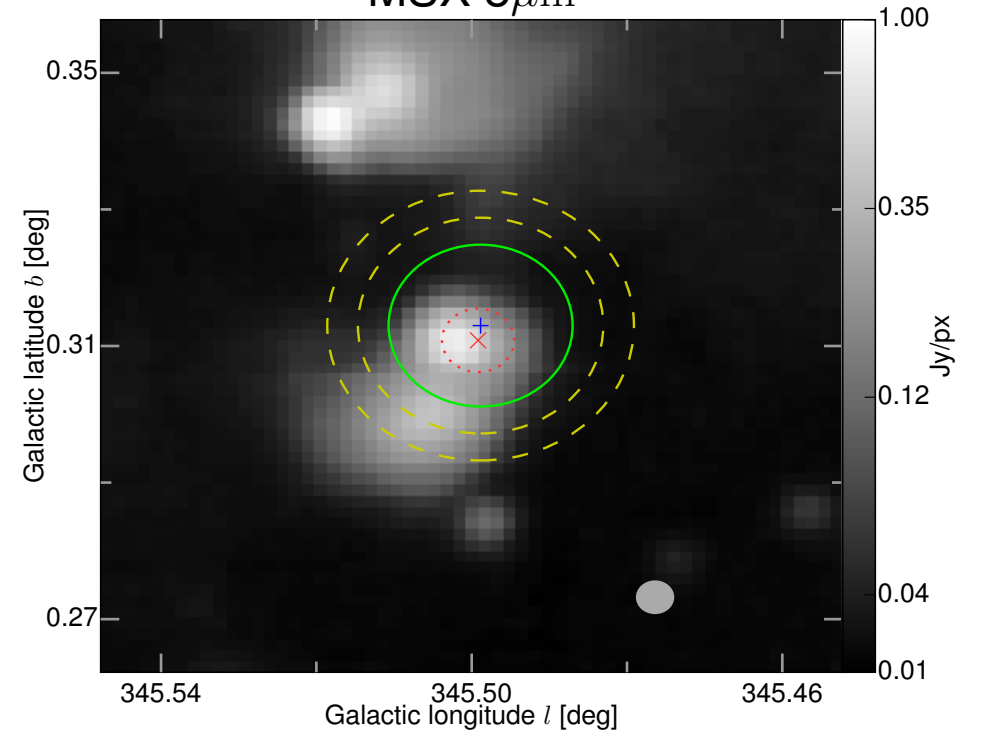
MSX 8 \mu\text{m}
