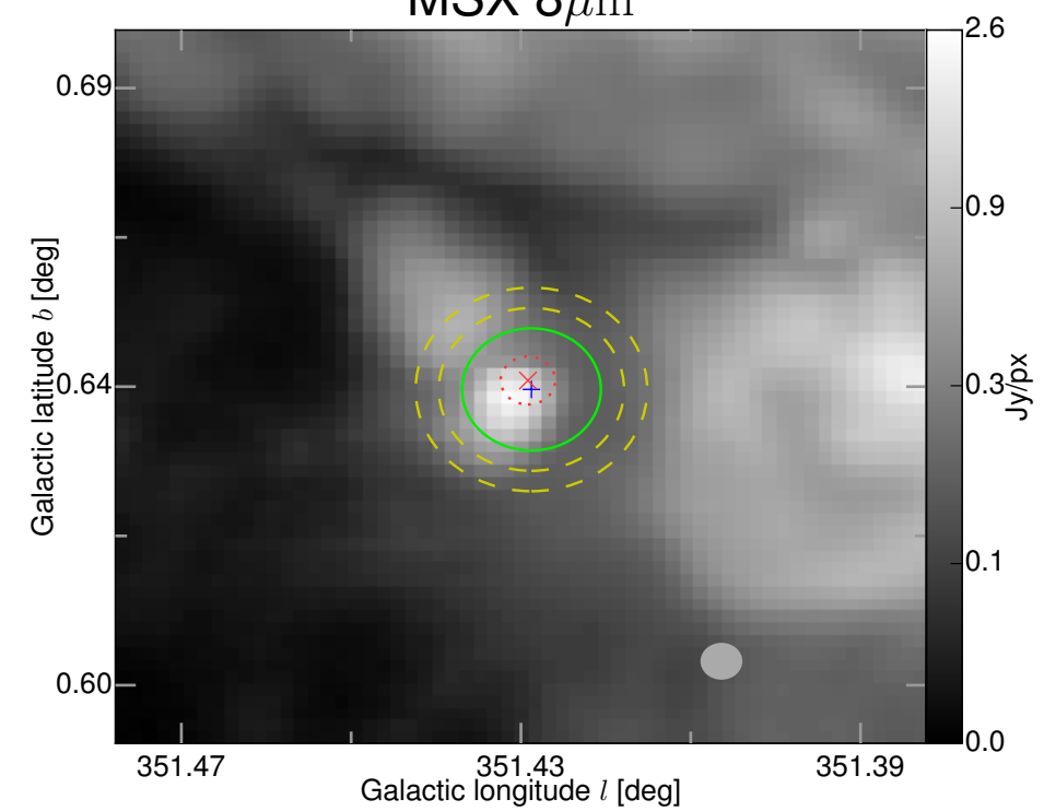
MSX 8\mu\text{m}
