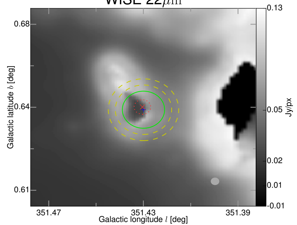
WISE 22\mu\text{m}
