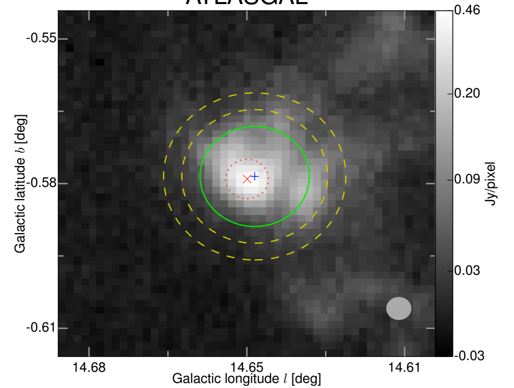
ATLASGAL
