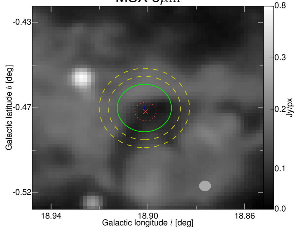
MSX 8\mu\text{m}
