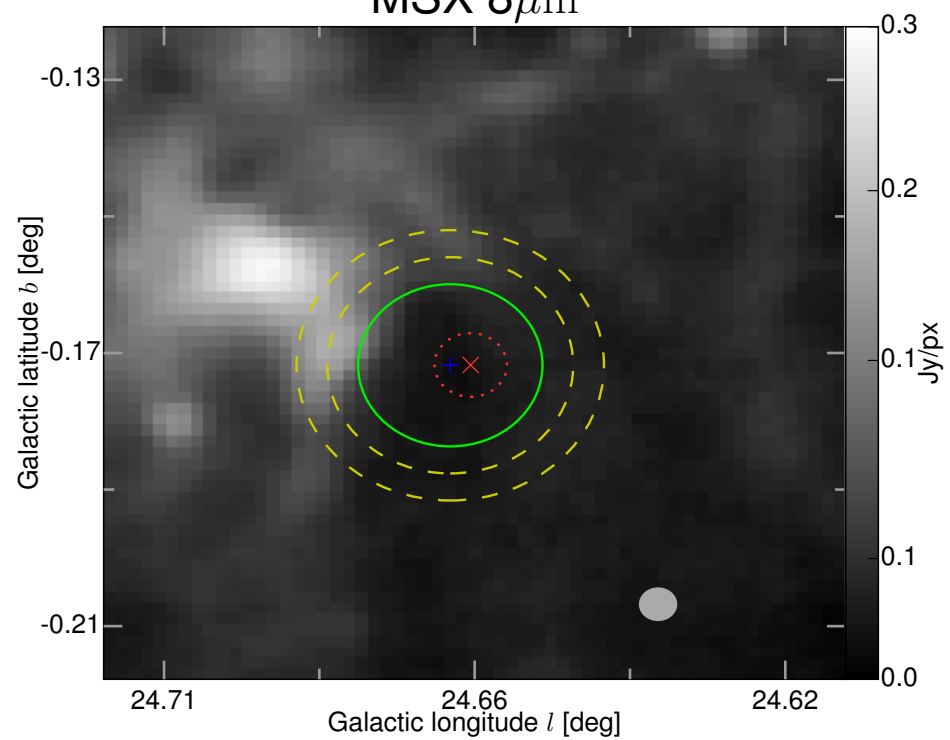
MSX 8 \mu\text{m}
