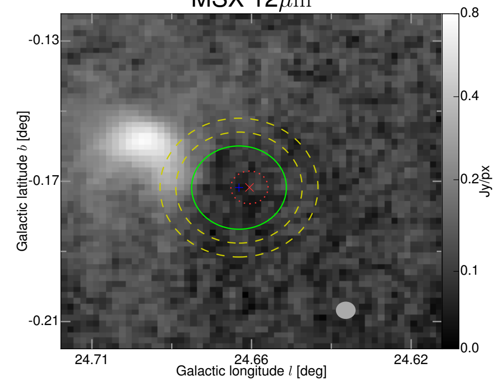
MSX 12 \mu\text{m}
