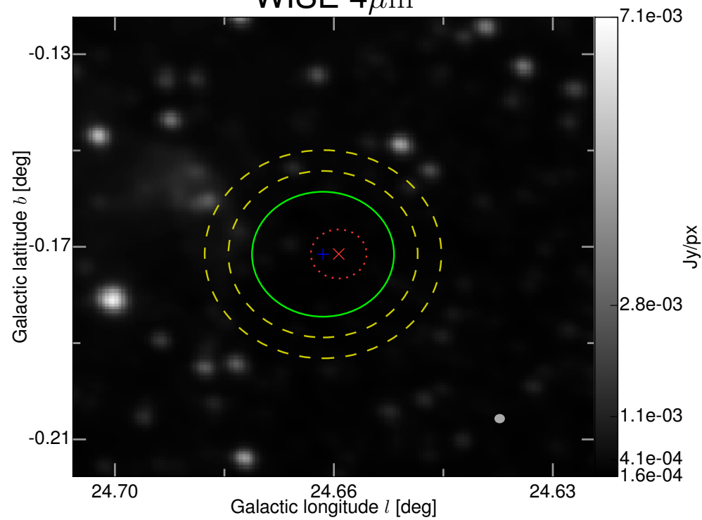
WISE 4 \mu\text{m}
