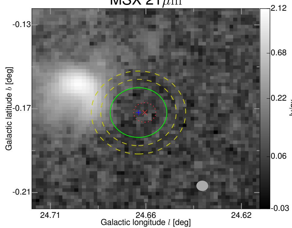
MSX 21 \mu\text{m}
