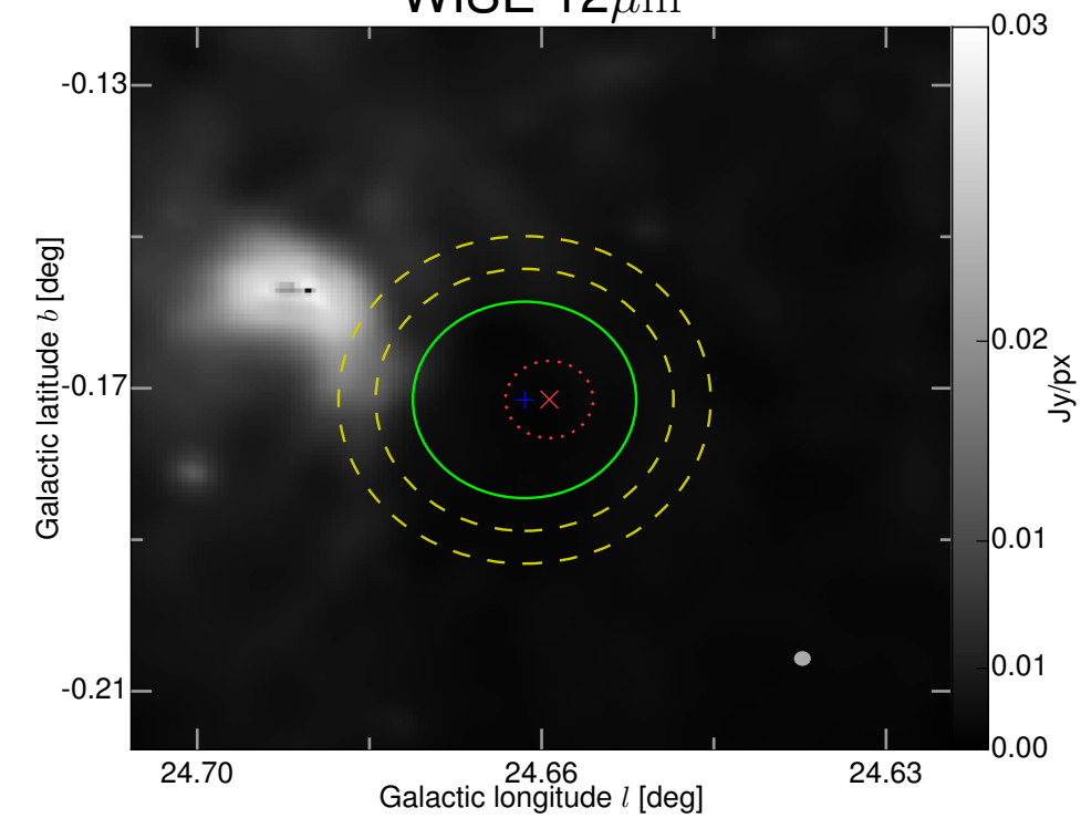
WISE 12 \mu\text{m}
