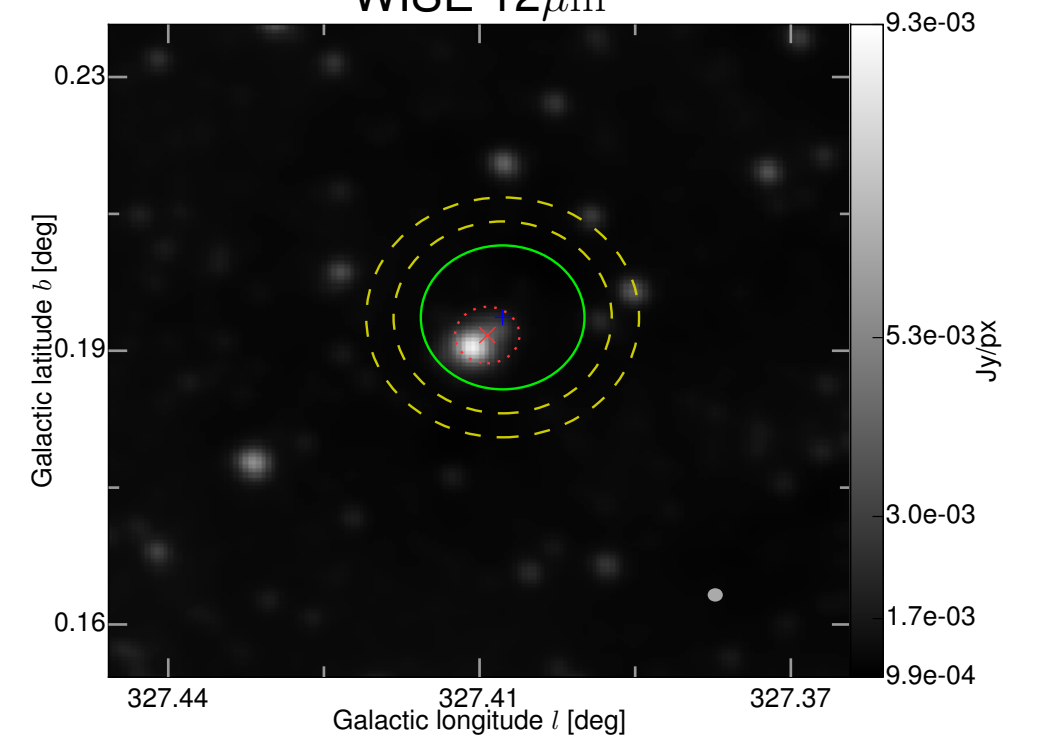
WISE 12\mu\text{m}
