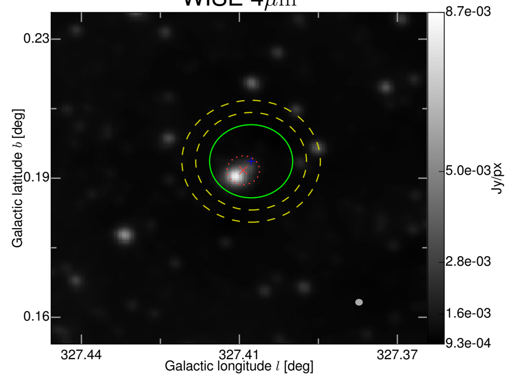
WISE 4\mu\text{m}
