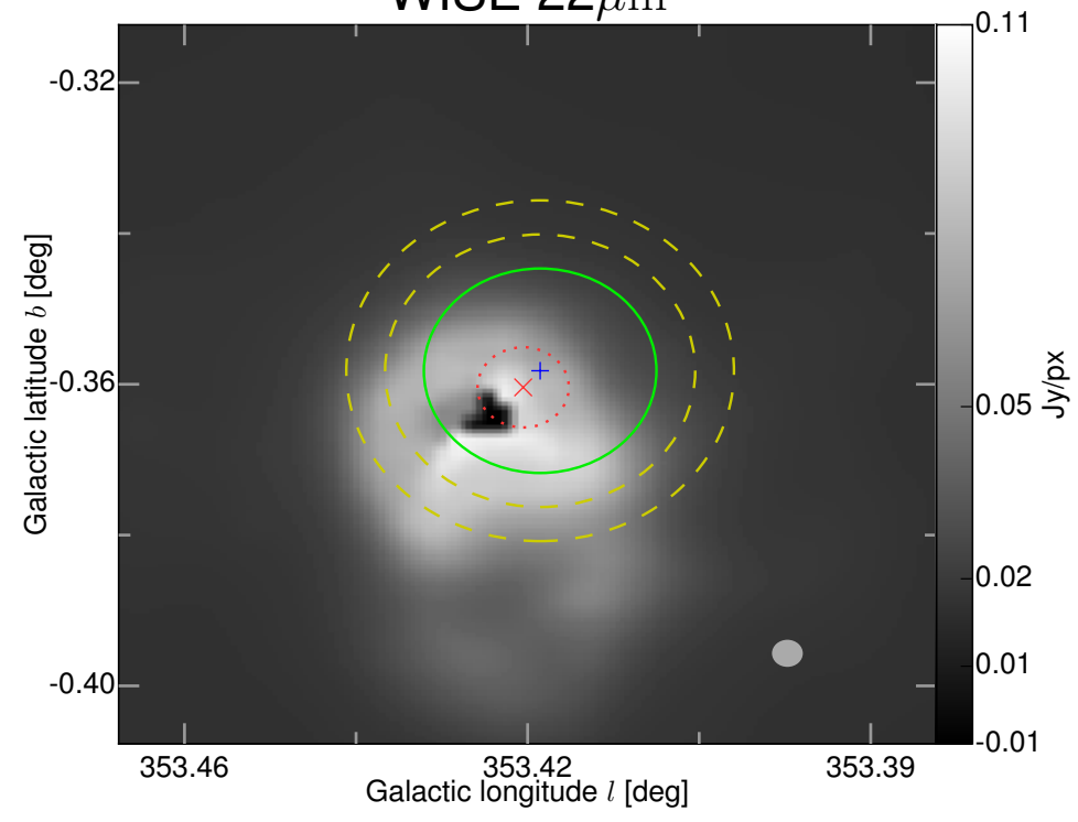
WISE 22 \mu m
