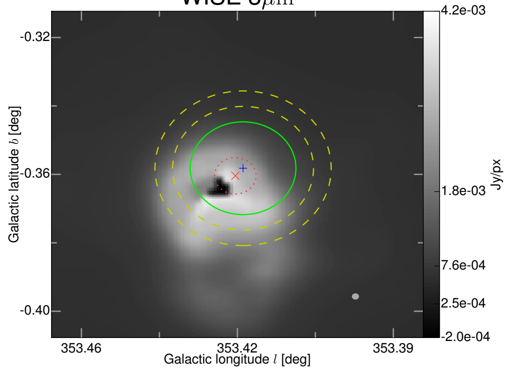
WISE 3 \mu m
