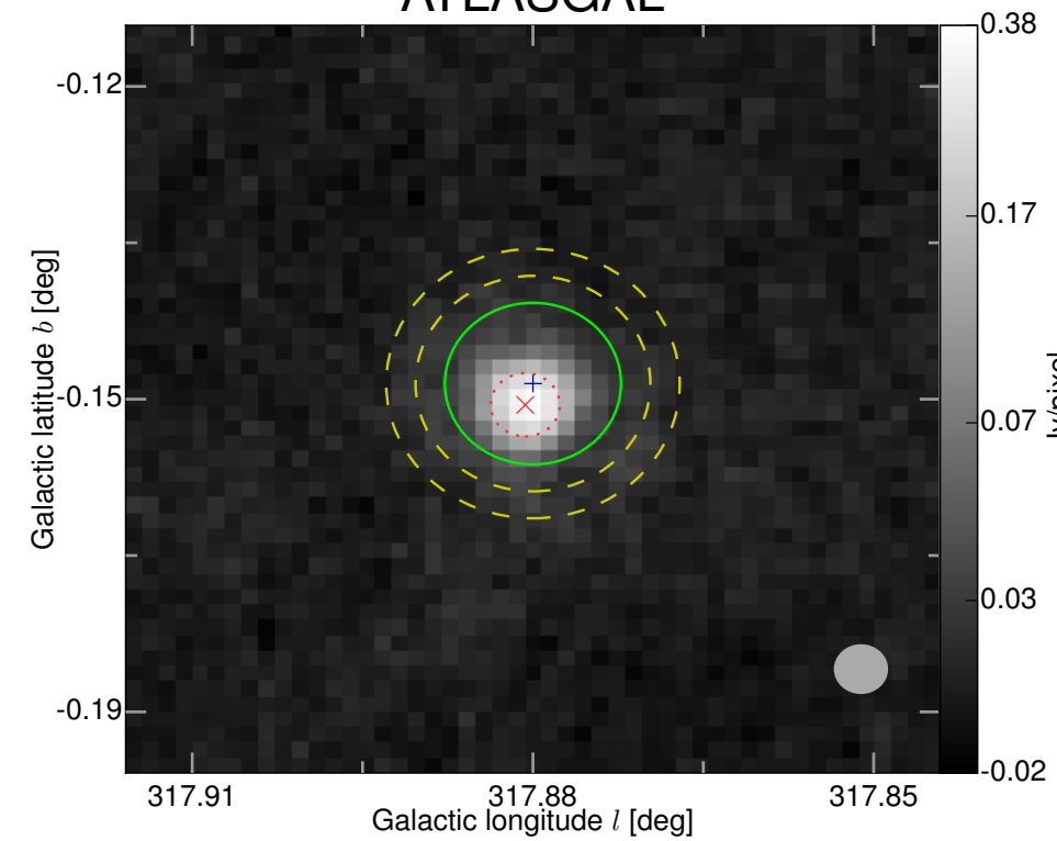
ATLASGAL
