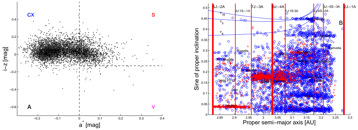
Figure 11. Panel A: an (a^*, i-z) projection of outer main belt asteroids in our multi-domain sample. Panel B: a (a, \sin(i)) projection of the same asteroids, where objects in the CX complex are shown as blue circles, and asteroids in the S-complex are identified as red plus signs.
