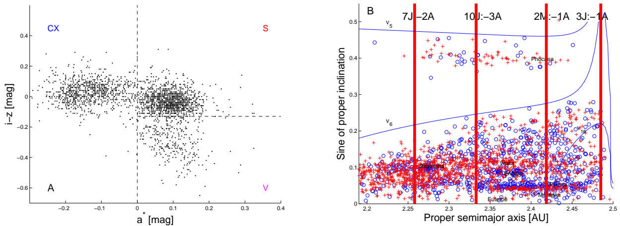
Figure 5. Panel A: an (a^*, i-z) projection of inner main belt asteroids in our multi-domain sample. Panel B: an (a, \sin(i)) projection of the same asteroids, where objects in the CX complex are shown as blue circles, and asteroids in the S-complex are identified as red plus signs.
