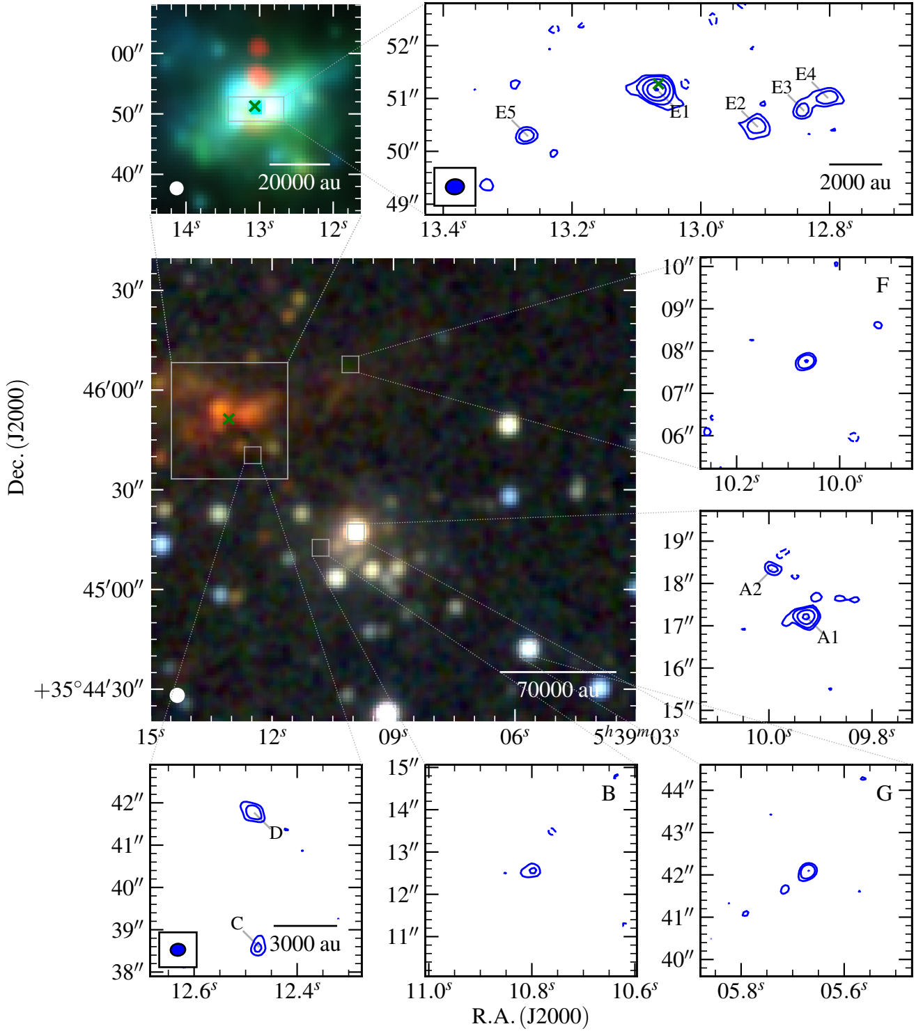
Figure B50. G173.4839+02.4317 - Near-infrared (R, G, B colour-scale, central, large panel; 2MASS, K, H, J bands), mid-infrared (R, G, B colour-scale, top left panel; GLIMPSE 8.0, 4.5, 3.6\mu\text{m} bands) and radio contour maps of G173.4839+02.4317 at C-band (other panels, blue contours). The restoring beam for the C-band data was 0.347'' \times 0.286'' at -84^\circ , while contour levels are set at (-3, 3, 5, 8, 14, 24) \times \sigma . All other values have the usual meaning. Green crosses show 6.7 GHz methanol maser positions from our data.
