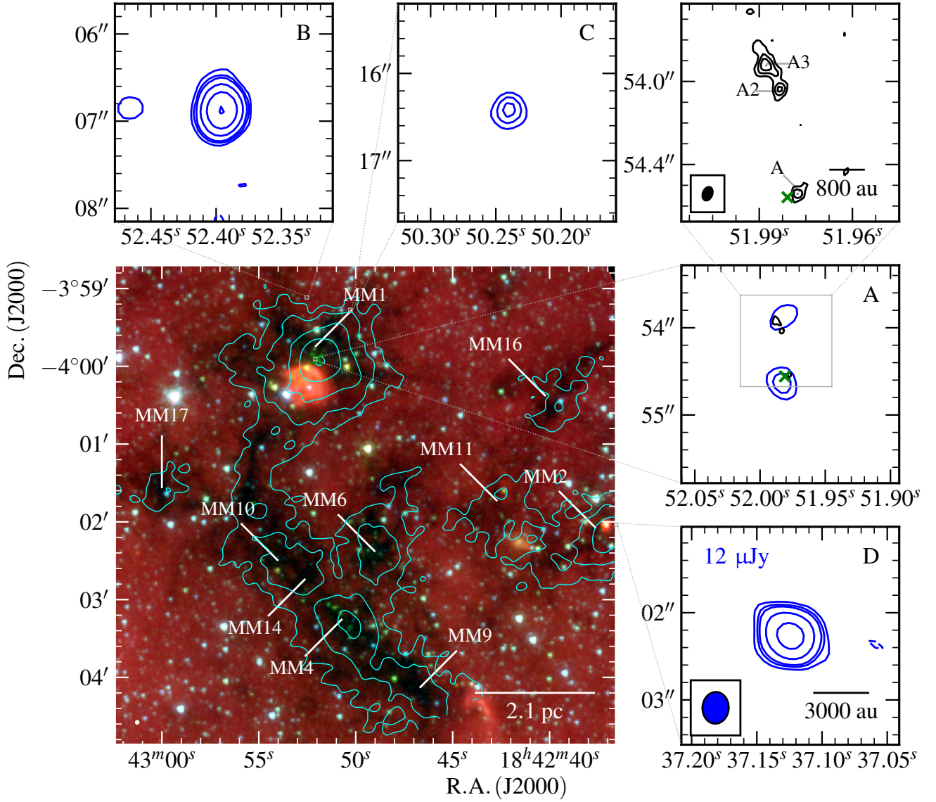
Figure B6. G028.37+00.07 - Mid-infrared (GLIMPSE 8.0, 4.5, 3.6μm R, G, B image; left panel), sub-mm (ATLASGAL 870μm cyan contours; left panel) and radio maps of G028.37+00.07 at C-band (blue contours; middle panels) and Q-band (black contours; right panel). Restoring beams were 0.364'' \times 0.301'' at -3^\circ and 0.068'' \times 0.046'' at -21^\circ , while contour levels are (-3, 3, 5, 7, 15, 34, 77) \times \sigma and (-3, 3, 5, 7, 9) \times \sigma for C and Q-band respectively, while ATLASGAL contours are set at (-3, 3, 6, 13, 28, 59) \times \sigma where \sigma = 87 mJy/beam. All other symbols/values have the usual meaning. Green crosses show 6.7 GHz methanol maser positions from our data.
