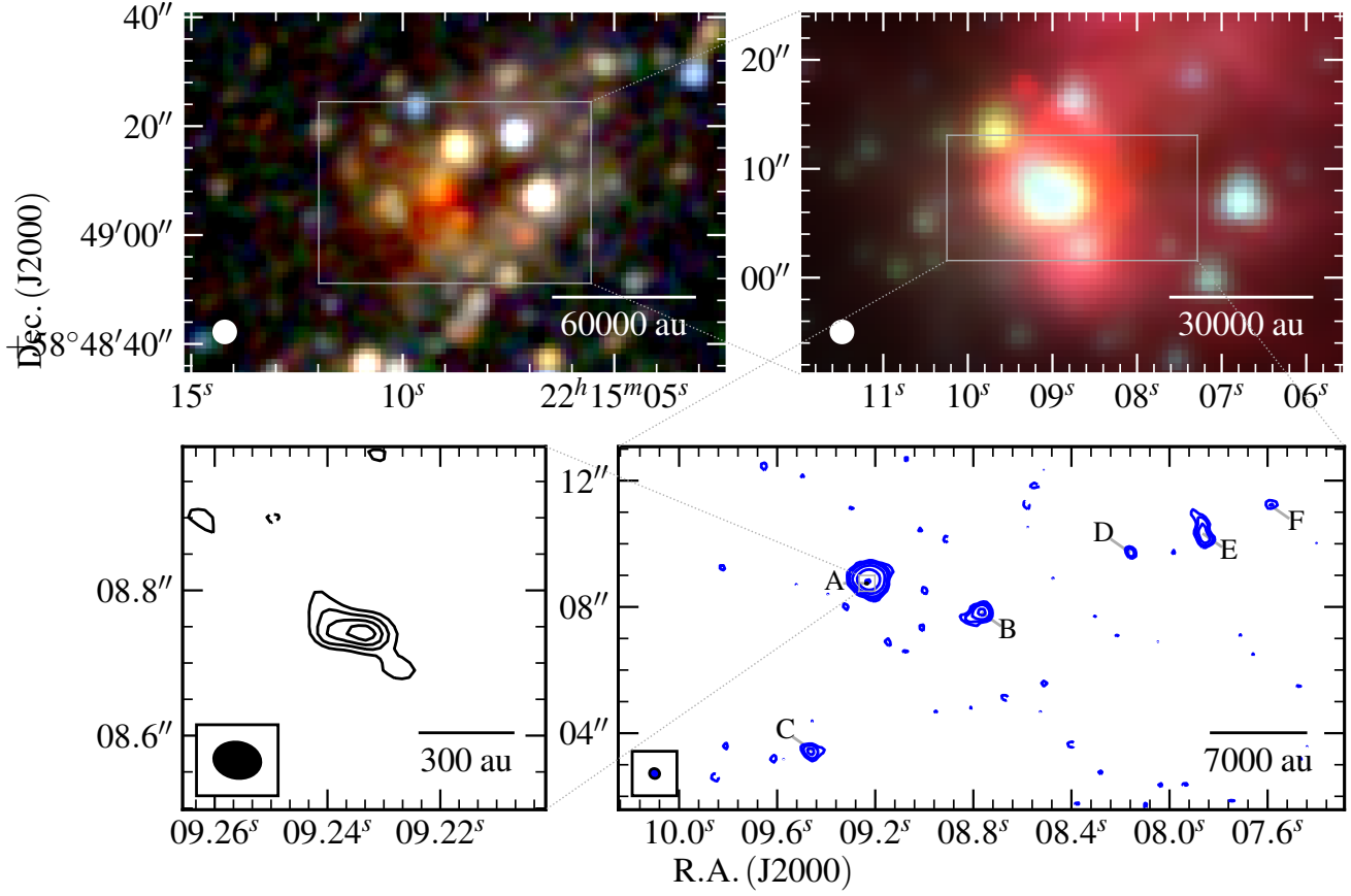
Figure B26. G103.8744+01.8558 - Mid-infrared (top right panel; GLIMPSE, 8.0, 4.5, 3.6 \mu m R, G, B colour-scale), near-infrared (top left panel; 2MASS, K, H, J, R, G, B colour-scale) and radio maps of G103.8744+01.8558 at C-band (blue contours; bottom-right) and Q-band (black contours; bottom left). Restoring beams were 0.327'' \times 0.302'' at 54^\circ and 0.065'' \times 0.050'' at 80^\circ , while contour levels are (-3, 3, 5, 9, 24, 70, 199) \times \sigma and (-3, 3, 4, 5, 6) \times \sigma for C and Q-band (robustness of 2) respectively. All other symbols have their usual meanings.
