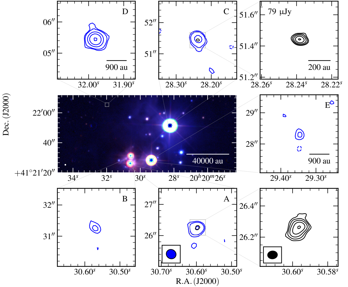
Figure B15. G078.8699+02.7602 - Near-infrared (middle row, left panel; UKIDSS, K, H, J, R, G, B colour-scale) and radio maps of G078.8699+02.7602 at C-band (blue contours; middle row and top right panels) and Q-band (black contours; bottom panels). Restoring beams were 0.319'' \times 0.295'' at 61^\circ and 0.062'' \times 0.050'' at -85^\circ for the C and Q-band data respectively. Contour levels are (-3, 3, 6, 16, 35, 80) \times \sigma for C-band images, (-3, 3, 5, 10, 20, 37) \times \sigma for the Q-band image of A and (-3, 3, 5, 8, 12, 19) \times \sigma for the Q-band image of C (due to varying noise across the primary beam). All other symbols/values have the usual meaning.
