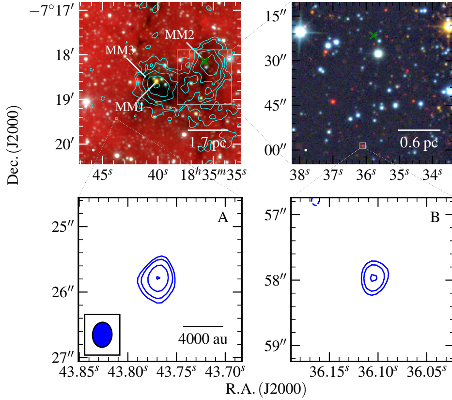
Figure B4. G024.60+00.08 - Mid-infrared (GLIMPSE 8.0, 4.5, 3.6 \mu\text{m} R, G, B image; top left panel), near-infrared (top right panel; UKIDSS, K, H, J bands in R, G, B colour-scale), sub-mm (ATLASGAL 870 \mu\text{m} cyan contours; top left panel) and C-band (blue contours; bottom panels) images of the IRDC, G024.60+00.08. The C-band restoring beam was 0.382'' \times 0.297'' at -4^\circ . C-band contour levels are (-3, 3, 5, 10, 18) \times \sigma and ATLASGAL contours are set at (-3, 3, 5, 8, 14, 24) \times \sigma where \sigma = 69 mJy/beam. All other values have their usual meaning. Green crosses show 6.7 GHz methanol maser positions from our data.
