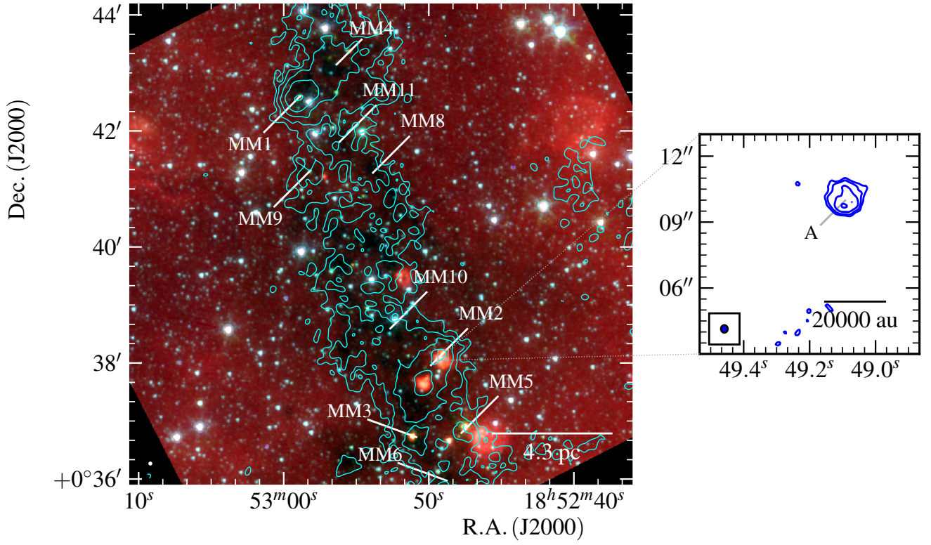
Figure B8. G033.69–00.01 - Mid-infrared (GLIMPSE 8.0, 4.5, 3.6 μm R, G, B image; left panel), sub-mm (ATLASGAL 870 μm cyan contours; left panel) and C-band radio map of G033.69–00.01 MM2 (right panel). The restoring beams used was 0.445'' \times 0.364'' at -53^\circ , while contour levels are set to (-4, 4, 7, 13, 22) \times \sigma , while ATLASGAL contours are set at (-3, 3, 5, 9, 15, 25) \times \sigma where \sigma = 85 mJy/beam. All other symbols/values have the usual meaning.
