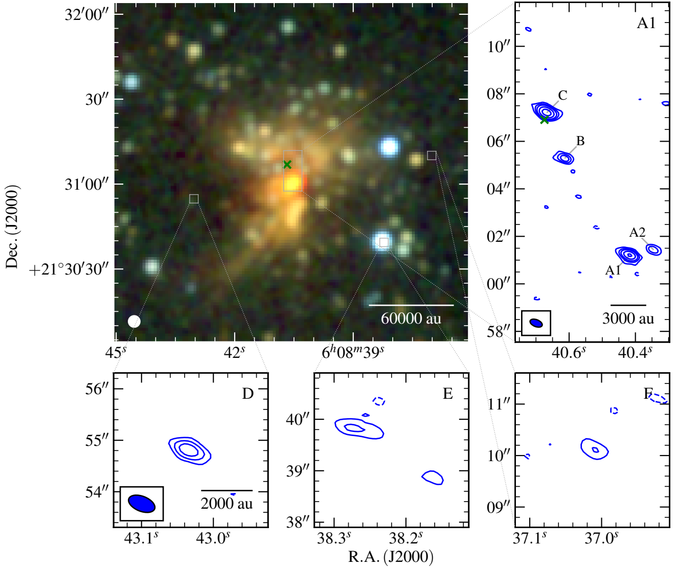
Figure B55. G189.0307+00.7821 - Near-infrared (R, G, B colour-scale, top left panel; 2MASS, K, H, J bands) and C-band (blue contours; bottom and top right panels) images of G189.0307+00.7821. The C-band restoring beam was 0.539'' \times 0.291'' at 68^\circ . Contour levels are (-3, 3, 6, 10, 19, 34) \times \sigma and all other values have their usual meaning. Green crosses show 6.7 GHz methanol maser positions from our data.
