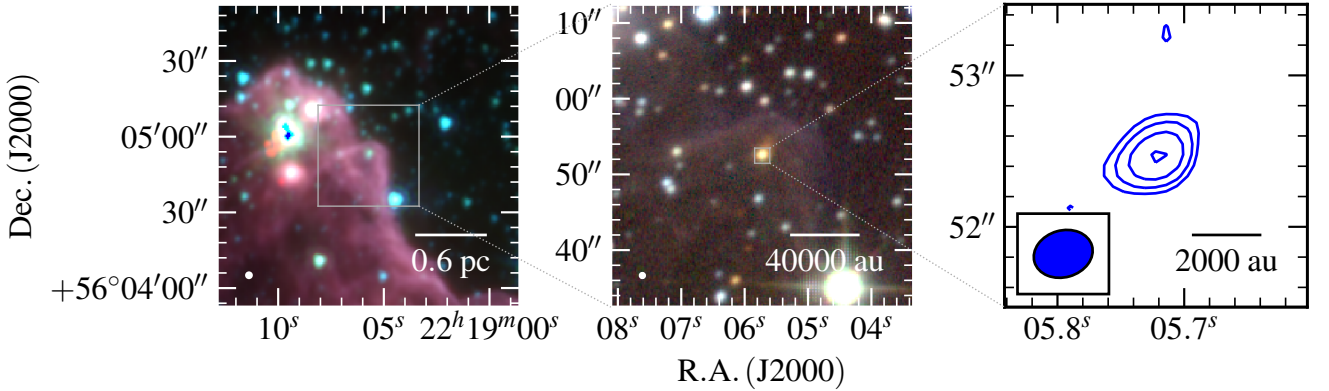
Figure B25. G102.8051–00.7184 - Mid-infrared (left panel; GLIMPSE, 8.0, 4.5, 3.6 \mu m R, G, B colour-scale), near-infrared (middle panel; UKIDSS, K, H, J bands in R, G, B colour-scale) and C-band radio map of G102.8051–00.7184 (right panel). The restoring beams used was 0.395'' \times 0.309'' at -75^\circ . Contour levels are (-3, 3, 5, 9, 14) \times \sigma . All other symbols/values have the usual meaning.
