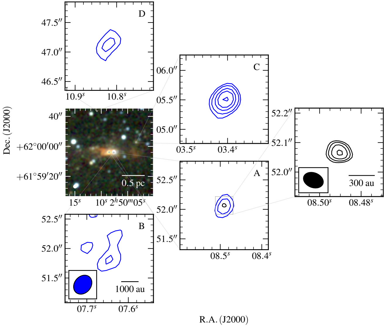
Figure B43. G136.3833+02.2666 - Near-infrared (R, G, B colour-scale, left panel; 2MASS, K, H, J bands) and radio contour maps of G136.3833+02.2666 at C-band (top left, bottom left and middle panels, blue contours) and Q-band (right panel, black contours). Restoring beams were 0.349'' \times 0.279'' at -40^\circ and 0.070'' \times 0.050'' at 69^\circ utilising a robustness of 2 for the Q-band data. Contour levels are (-3, 3, 5, 9, 13, 20) \times \sigma and (-3, 3, 4, 6, 9) \times \sigma for C and Q-band respectively. Varying noises across the C-band primary beam are represented. All other values have the usual meaning.
