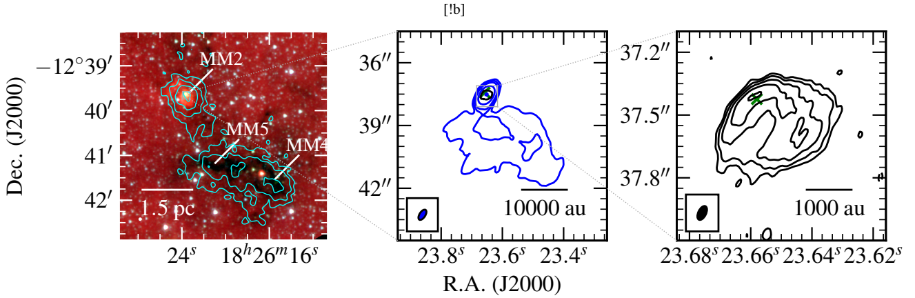
Figure B1. G018.82–00.28 - Mid-infrared (GLIMPSE 8.0, 4.5, 3.6 \mu m R, G, B image; left panel), sub-mm (ATLASGAL 870 \mu m cyan contours; left panel) and radio maps of G018.82–00.28 at C-band (blue contours; middle) and Q-band (black contours; right). Restoring beams were 0.558'' \times 0.283'' at -33^\circ and 0.072'' \times 0.038'' at -26^\circ , while contour levels are (-3, 3, 6, 12, 44, 171) \times \sigma and (-3, 3, 6, 11, 21, 40) \times \sigma for C and Q-band respectively and ATLASGAL contours are set at (-3, 3, 5, 9, 15) \times \sigma where \sigma = 82 mJy/beam. Green crosses show 6.7 GHz methanol maser positions from our data. In the infrared images, a white ellipse is used to denote the approximate PSF of the relevant instrument. All other symbols/values have the usual meaning. If RMS noises are displayed in a subplot, that is because in the location of the source the RMS noise diverges from that quoted in Table A1 .
