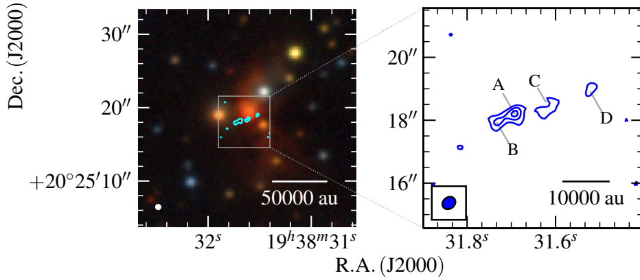
Figure B13. G056.3694–00.6333 - Near-infrared (left panel; UKIDSS, K, H, J bands in R, G, B colour-scale) and C-band radio map (robustness of 2) of G056.3694–00.6333 (right panel). The restoring beams used was 0.445'' \times 0.364'' at -53^\circ , while contour levels are set to (-3, 3, 5, 7) \times \sigma . All other symbols/values have the usual meaning. To highlight the slight offset between the reddened UKIDSS source and radio lobes, the radio 3\sigma contour is overlaid upon the NIR image (cyan).
