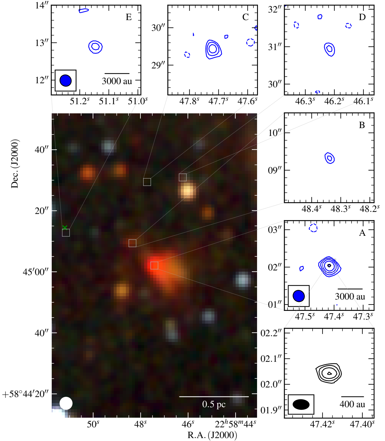
Figure B32. G108.7575–00.9863 - Mid-infrared (R, G, B colour-scale, left panel; 2MASS, K,H,J bands R, G, B colour-scale) and radio maps of G108.7575–00.9863 at C-band (blue contours; top and middle-right panels) and Q-band (black contours; bottom right). Restoring beams were 0.312'' \times 0.295'' at 44^\circ and 0.063'' \times 0.038'' at 88^\circ , while contour levels were set at (-3, 3, 5, 8, 12, 19) and (-3, 3, 5, 9, 15) \times \sigma for the C and Q-band (robustness of 2) data respectively. Varying noise levels are the result of missing spatial scale information leading to non-Gaussian noise and primary beam effects. Green crosses show 6.7 GHz methanol maser positions from our data.
