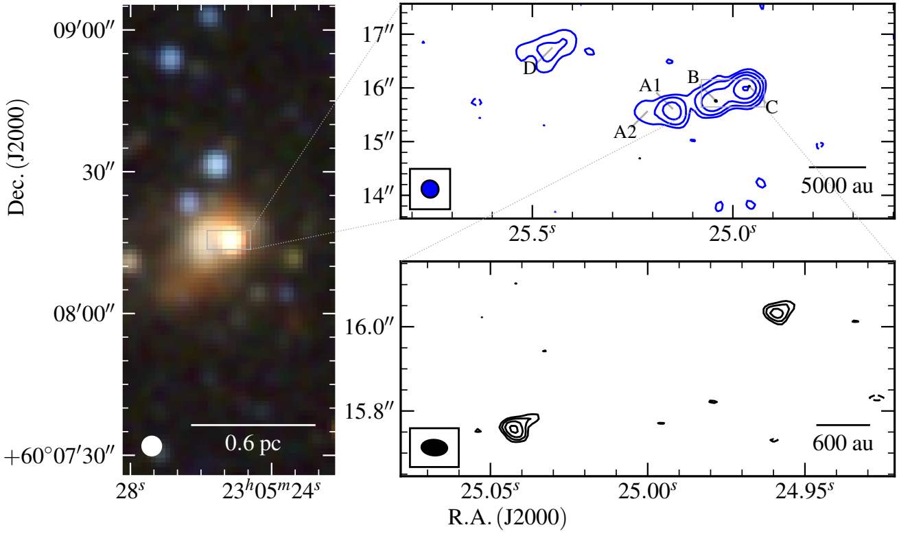
Figure B33. G110.0931–00.0641 - Near-infrared (R, G, B colour-scale, left panel; 2MASS, K, H, J bands ) and radio maps of the G110.0931–00.0641 field at C-band (blue contours; middle) and Q-band (black contours; right). Restoring beams were 0.326'' \times 0.314'' at 36^\circ and 0.063'' \times 0.038'' at 86^\circ , while contour levels are (-3, 3, 7, 14, 32, 69) \times \sigma and (-3, 3, 4, 5, 6) \times \sigma for C and Q-band respectively. All other symbols/values have the usual meaning.
