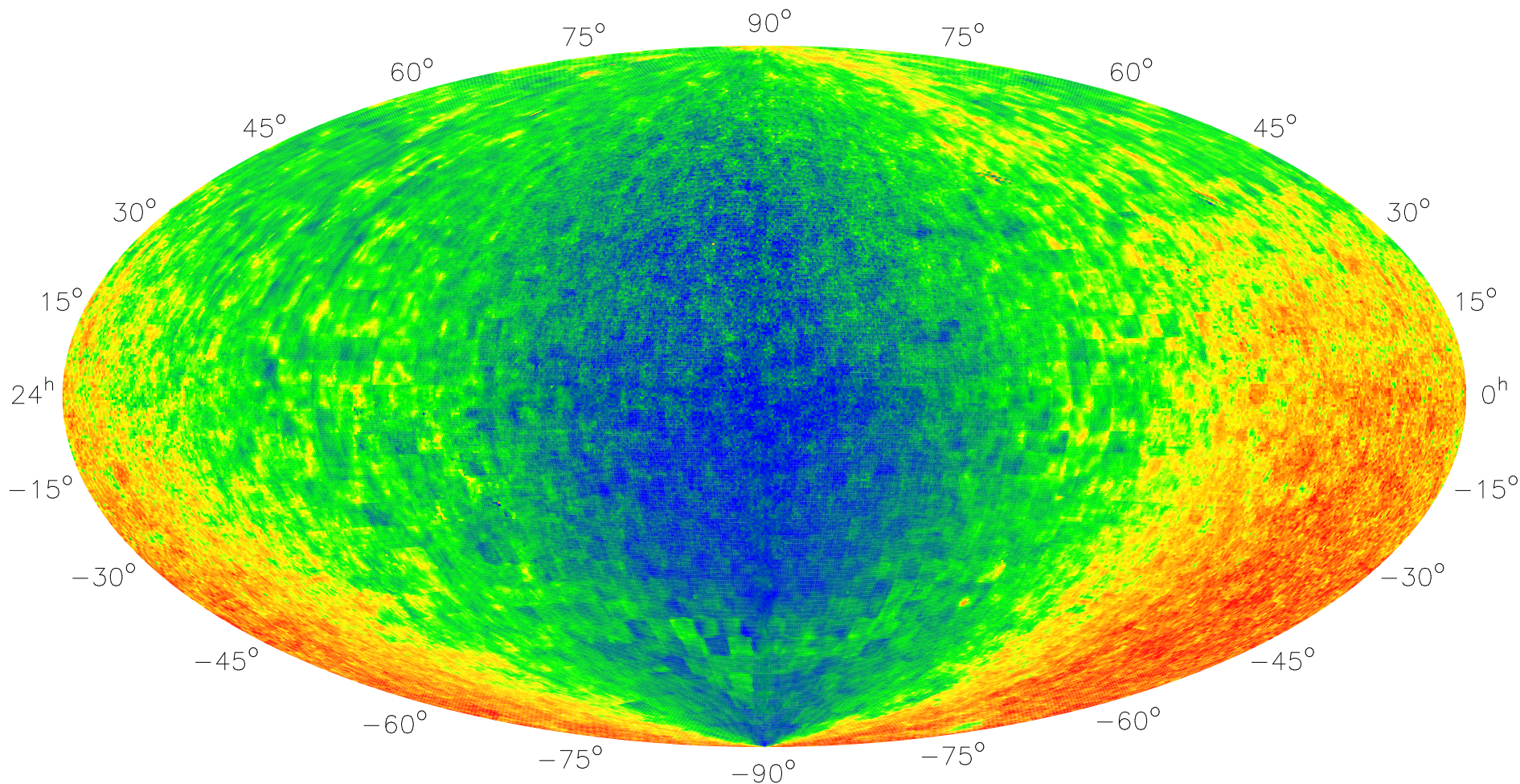
UCAC4 mean PM RAcosD [mas/yr]
