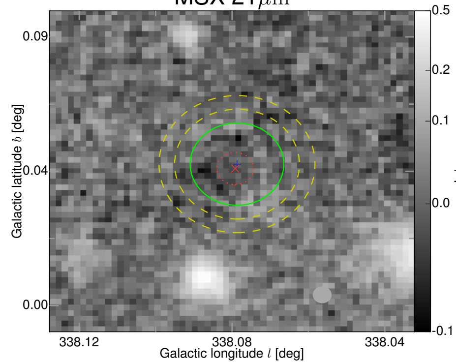
MSX 21\mu\text{m}
