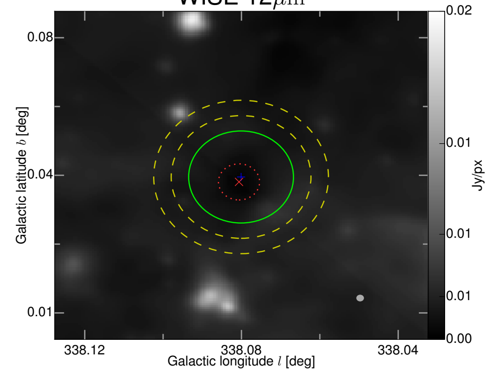
WISE 12\mu\text{m}
