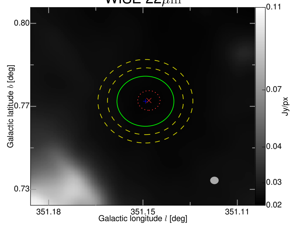
WISE 22\mu\text{m}
