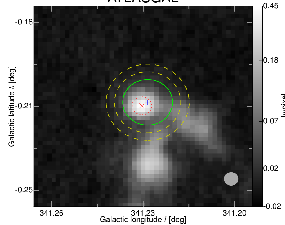
ATLASGAL
