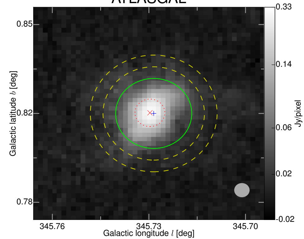
ATLASGAL
