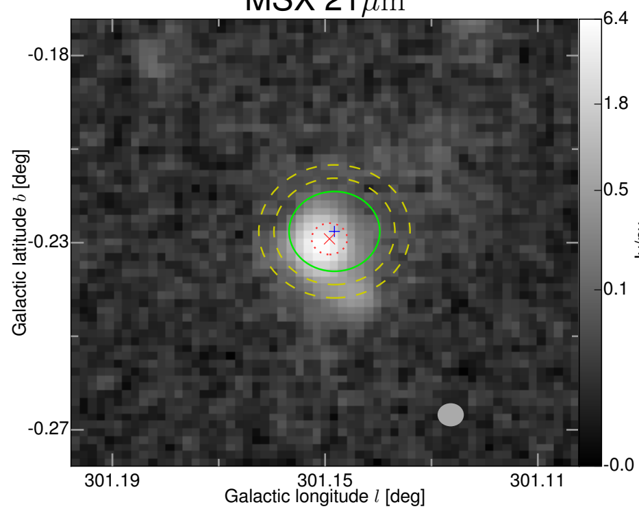
MSX 21\mu\text{m}
