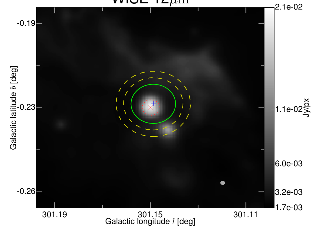
WISE 12\mu\text{m}
