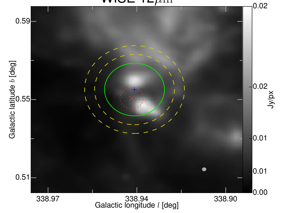
WISE 12\mu\text{m}
