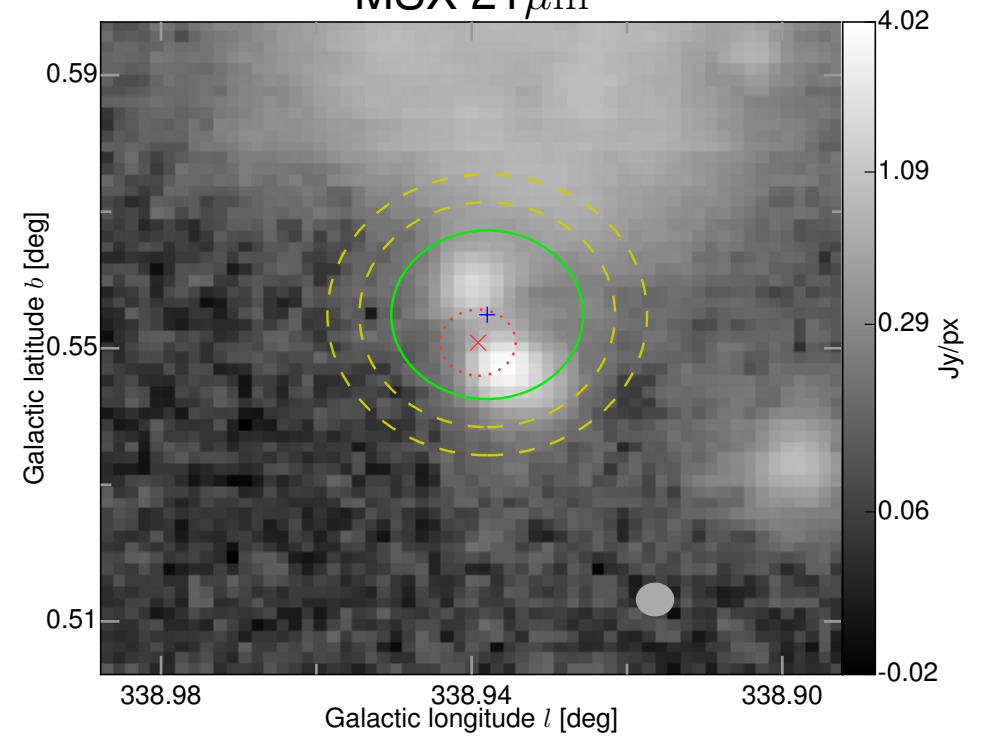
MSX 21\mu\text{m}
