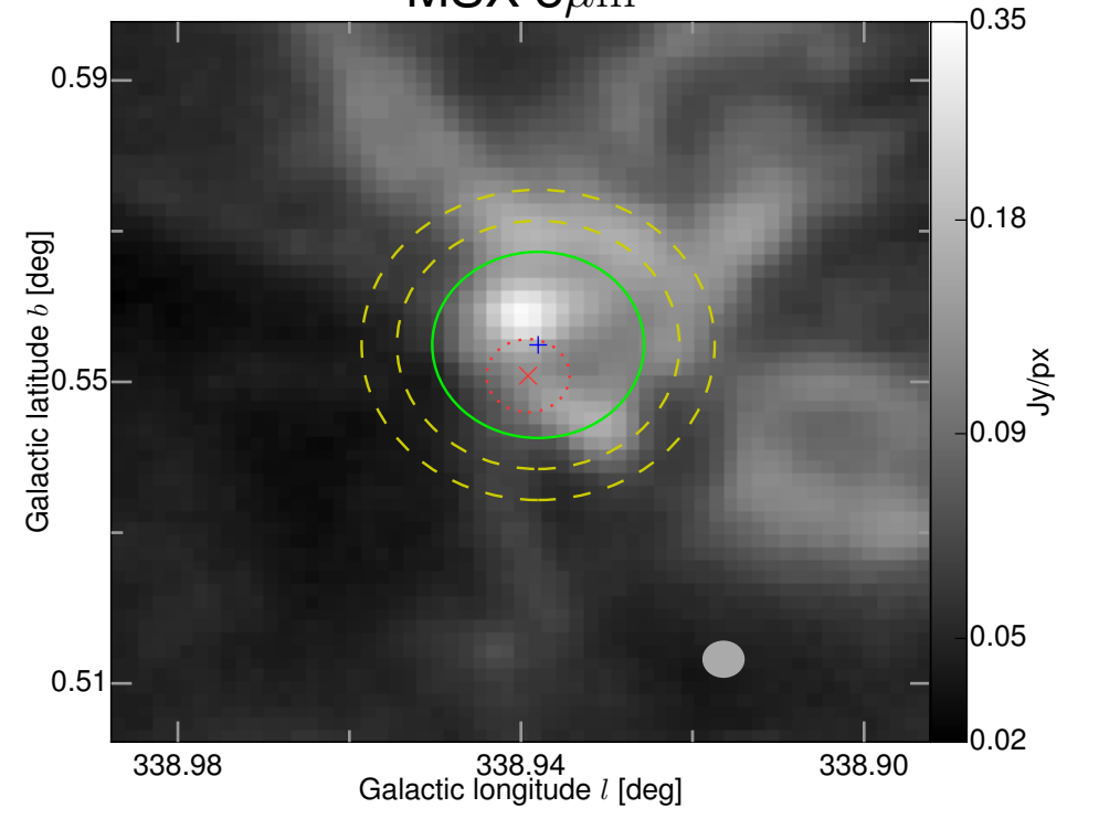
MSX 8\mu\text{m}
