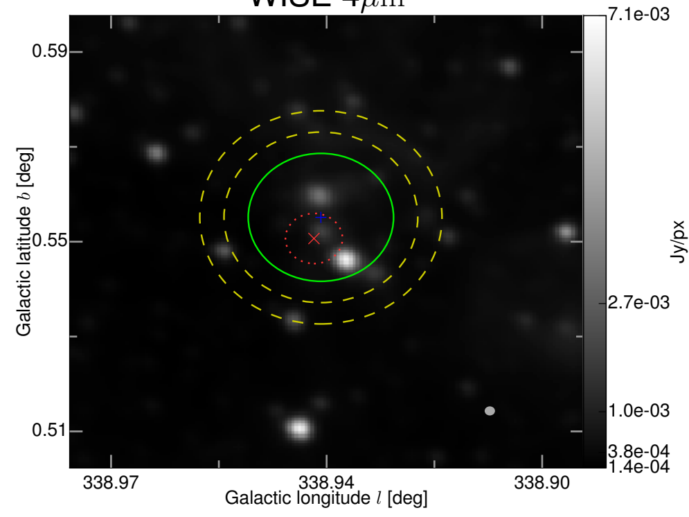
WISE 4\mu\text{m}
