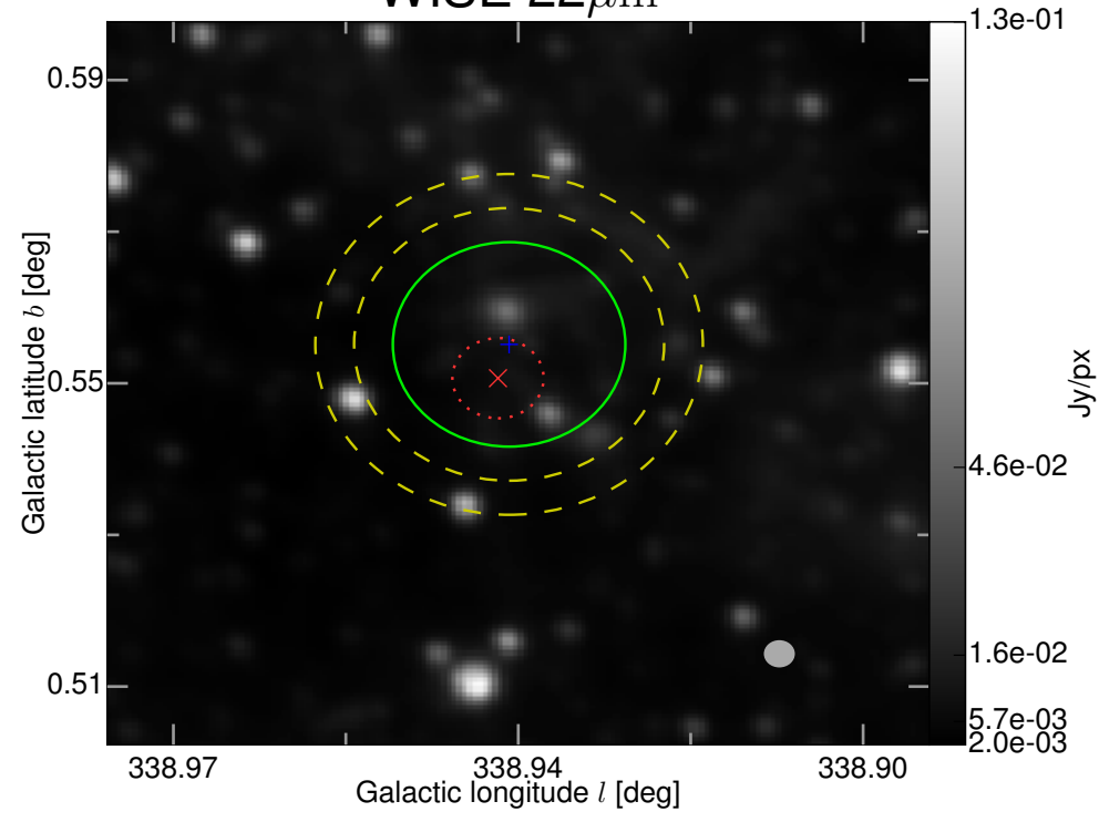
WISE 22\mu\text{m}
