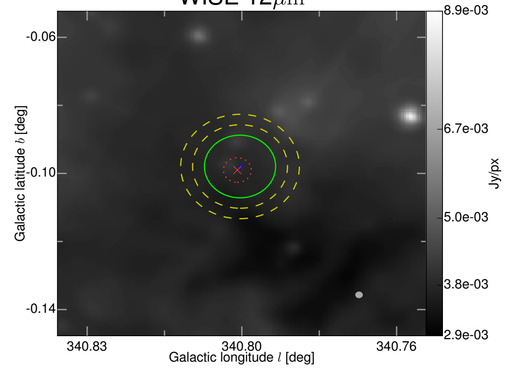
WISE 12\mu\text{m}
