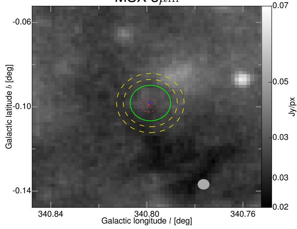
MSX 8\mu\text{m}
