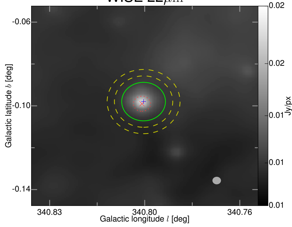
WISE 22\mu\text{m}
