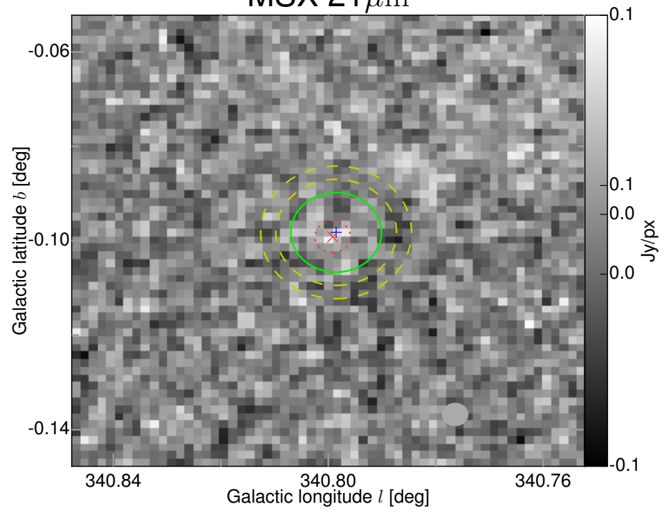
MSX 21\mu\text{m}
