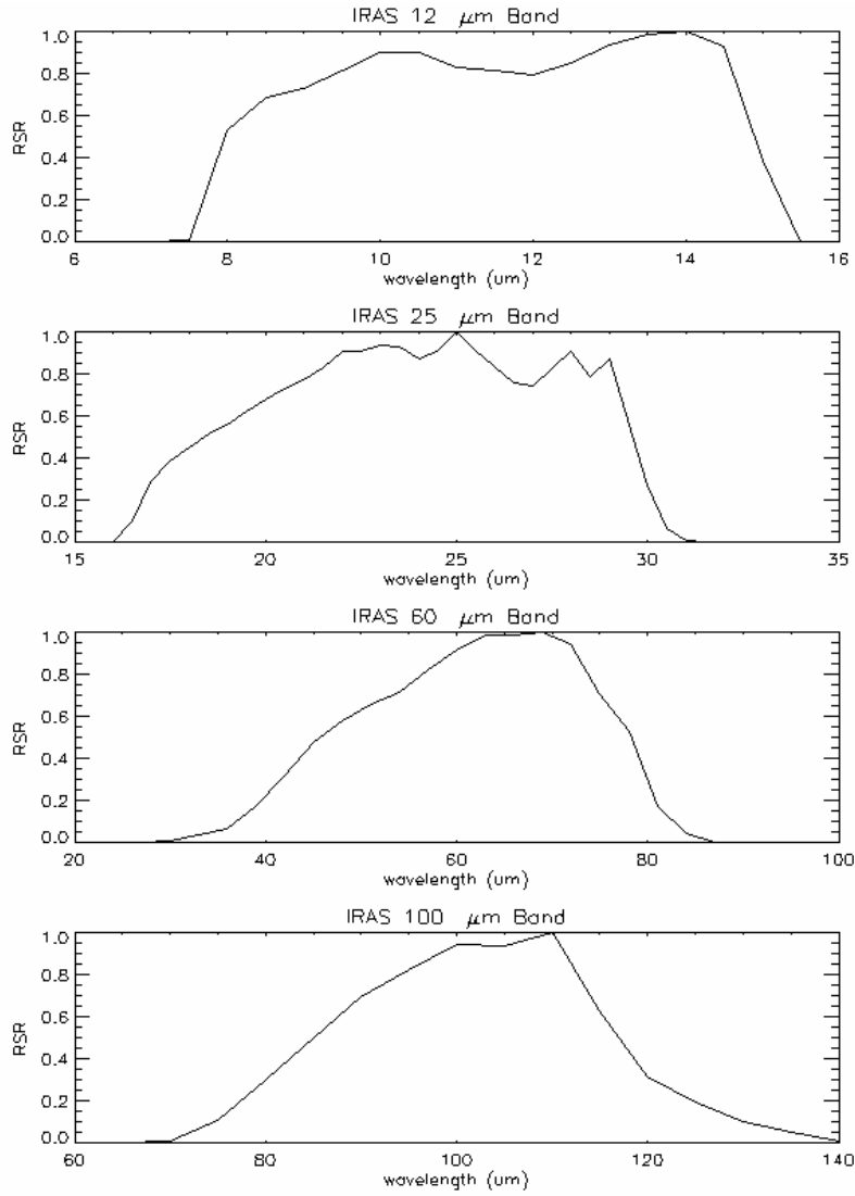
Figure C-1 IRAS Wavebands
