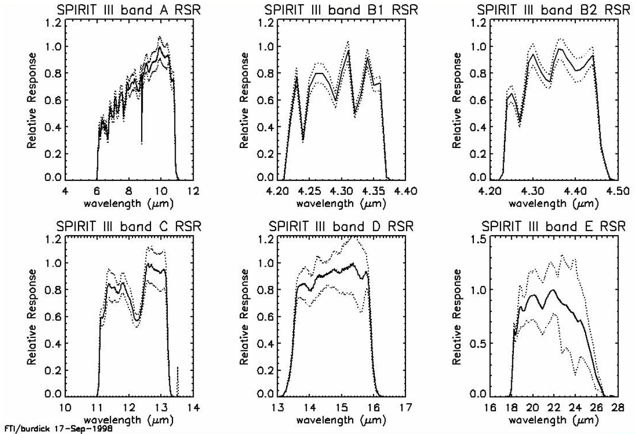
Figure A-1. SPIRIT III Radiometer Measured Relative Spectral Response (RSR)
