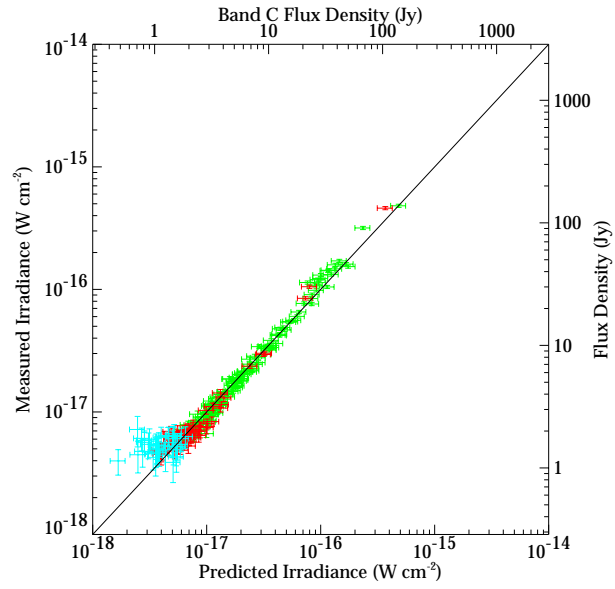
Figure 20: Band C measurements versus IRAS based predicted fluxes.
