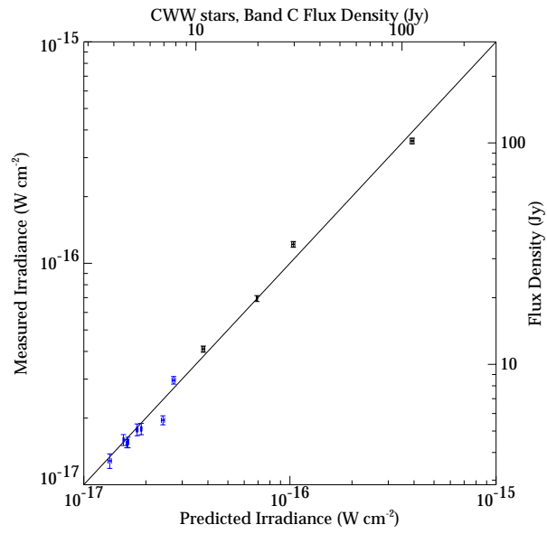
Figure 8: Band C calibration stars.
