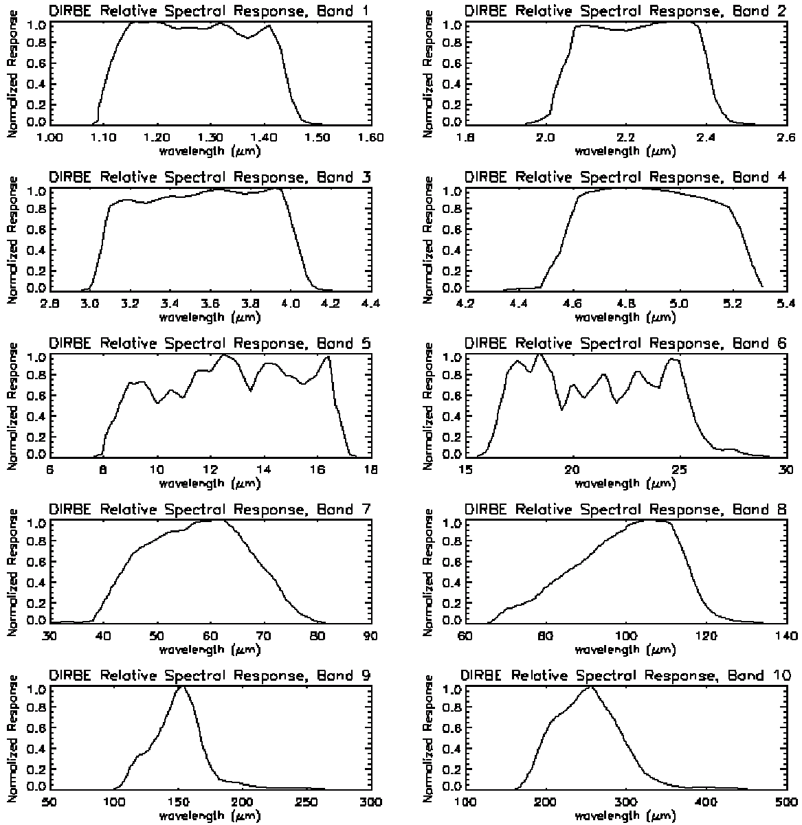
Figure C-2 DIRBE Wavebands
