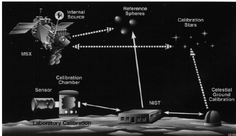
Figure 3: SPIRIT III calibration.
