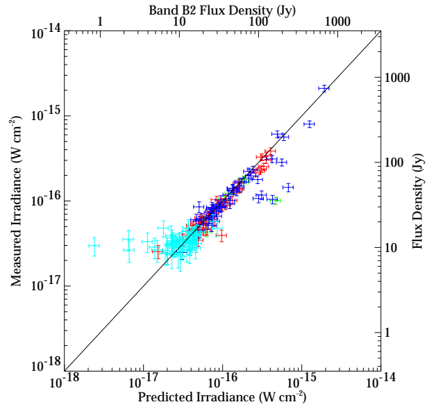
Figure 18: Band B 2 measurements versus IRAS based predicted fluxes.
