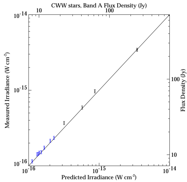
Figure 7: Band A calibration stars.
