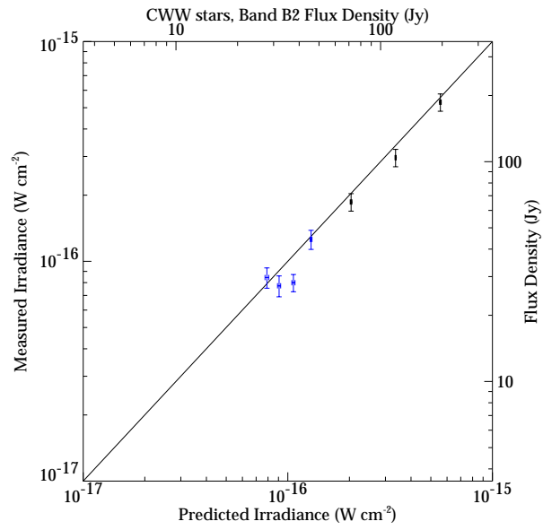
Figure 6: Band B 2 calibration stars.
