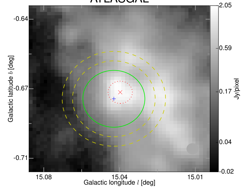
ATLASGAL
