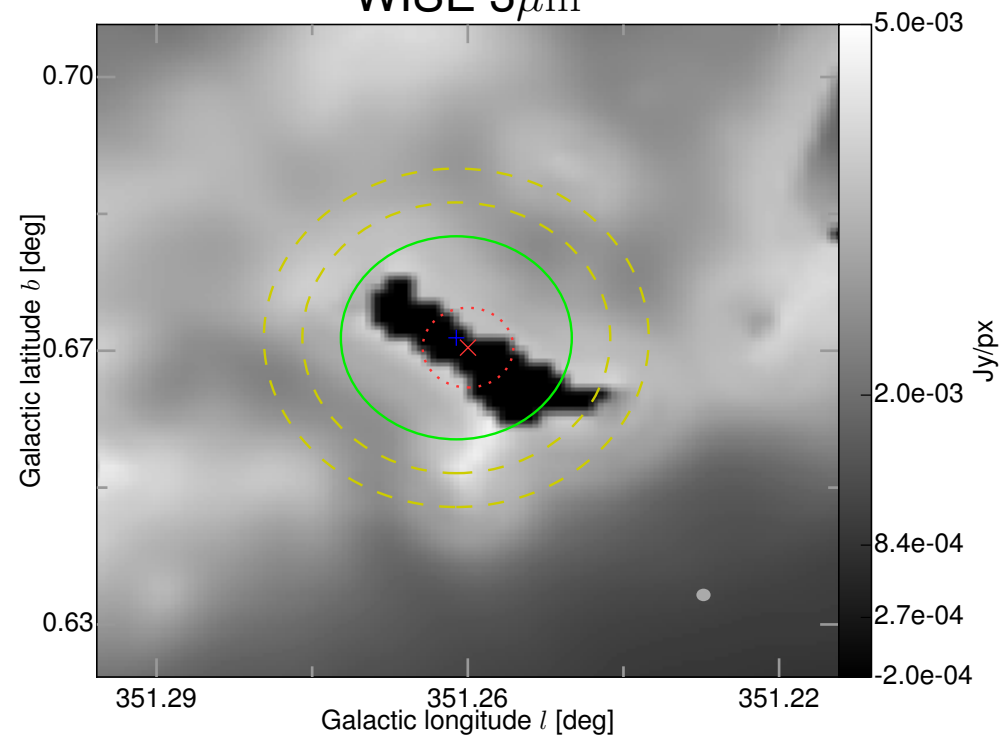
WISE 3 \mu\text{m}
