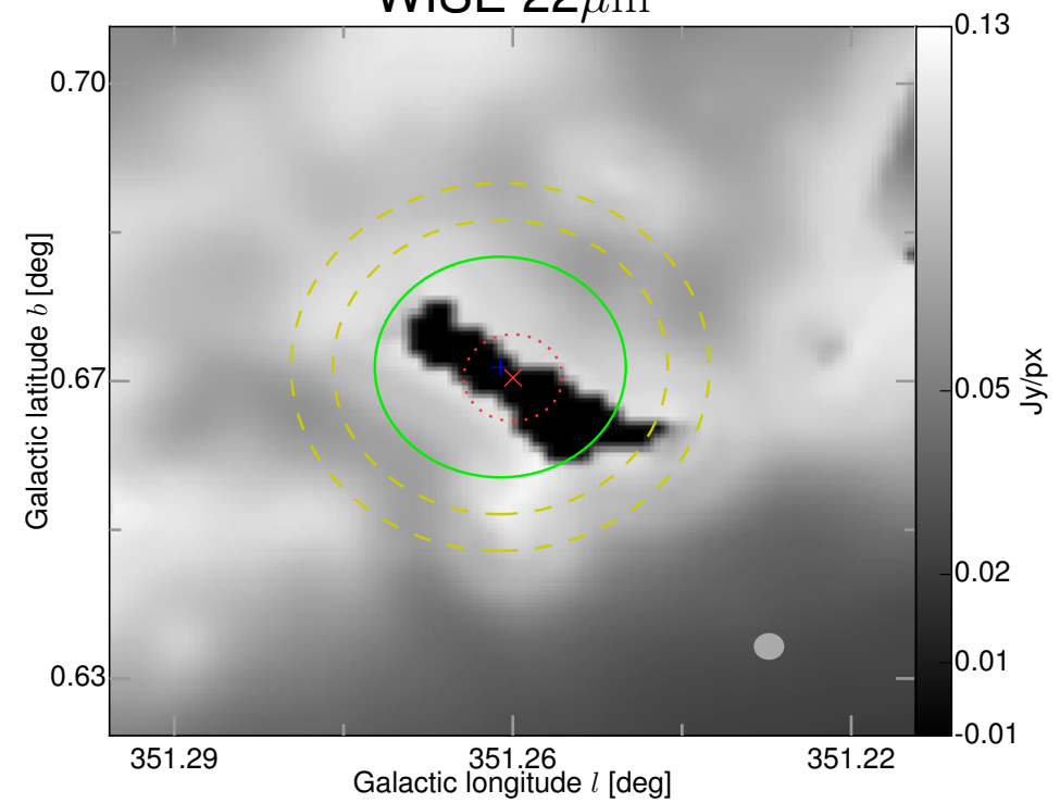
WISE 22 \mu\text{m}
