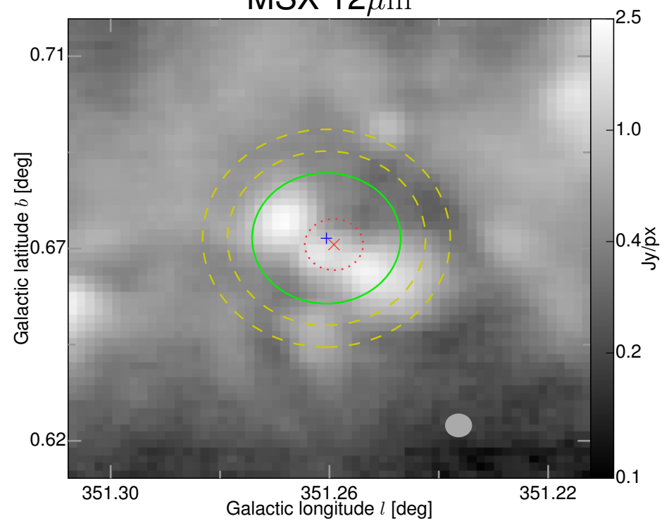
MSX 12 \mu\text{m}
