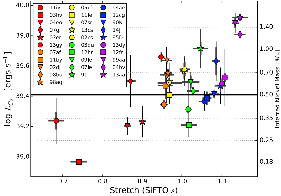
Figure 7. [\text{Co III}] \lambda 5893 line luminosity scaled to its equivalent value at t = 200 d using the M_{\text{Co}}(t)^2 curve ( L_{\text{Co}} ) versus SN light-curve stretch. As in Fig. 6, thick error bars correspond to flux measurement errors, while narrow error bars correspond to distance uncertainty arising from peculiar velocities.
