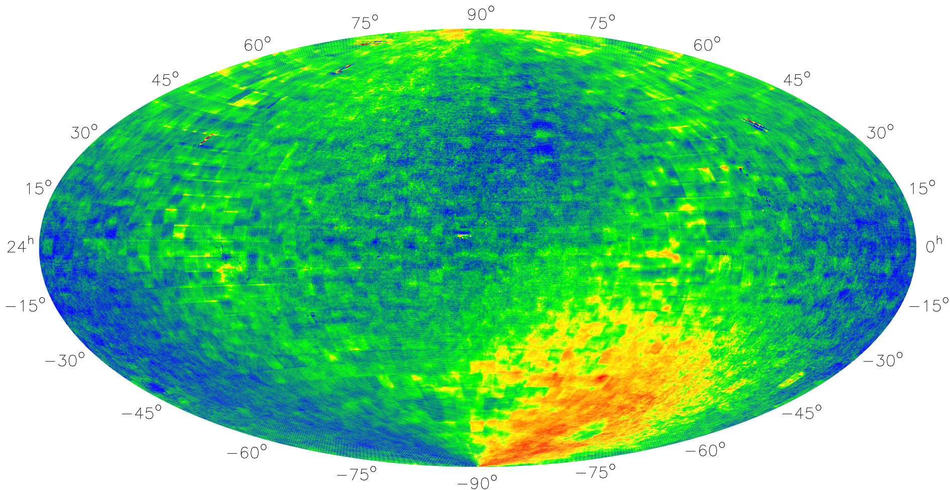
UCAC4 mean PM Dec [mas/yr]
