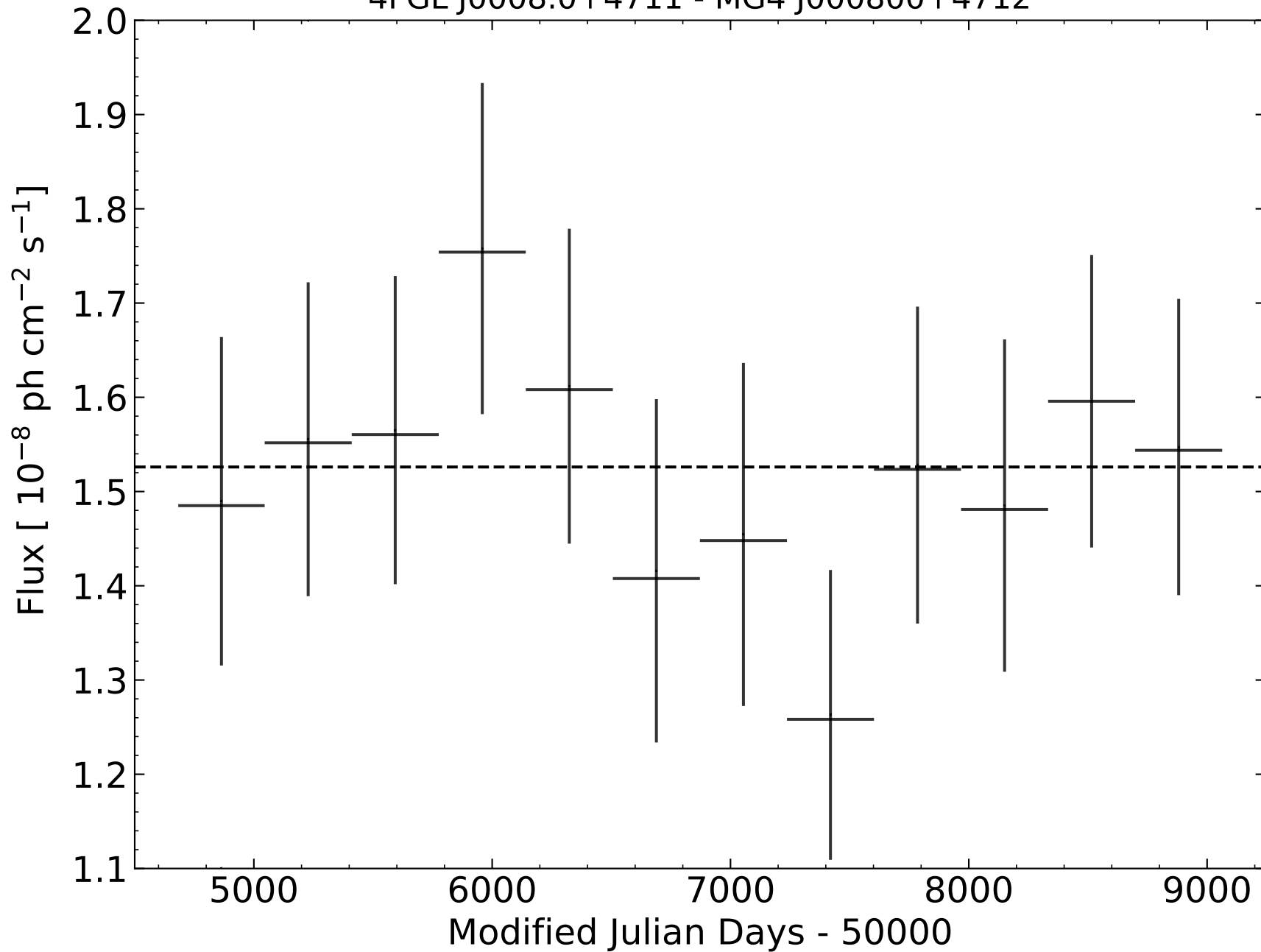
4FGL J0008.0+4711 - MG4 J000800+4712
