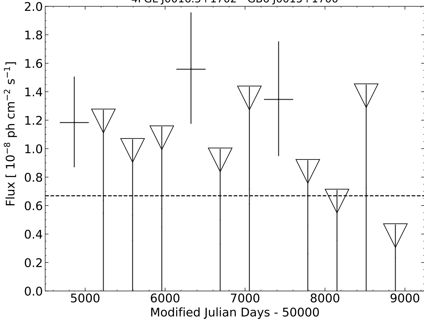
4FGL J0016.5+1702 - GB6 J0015+1700
