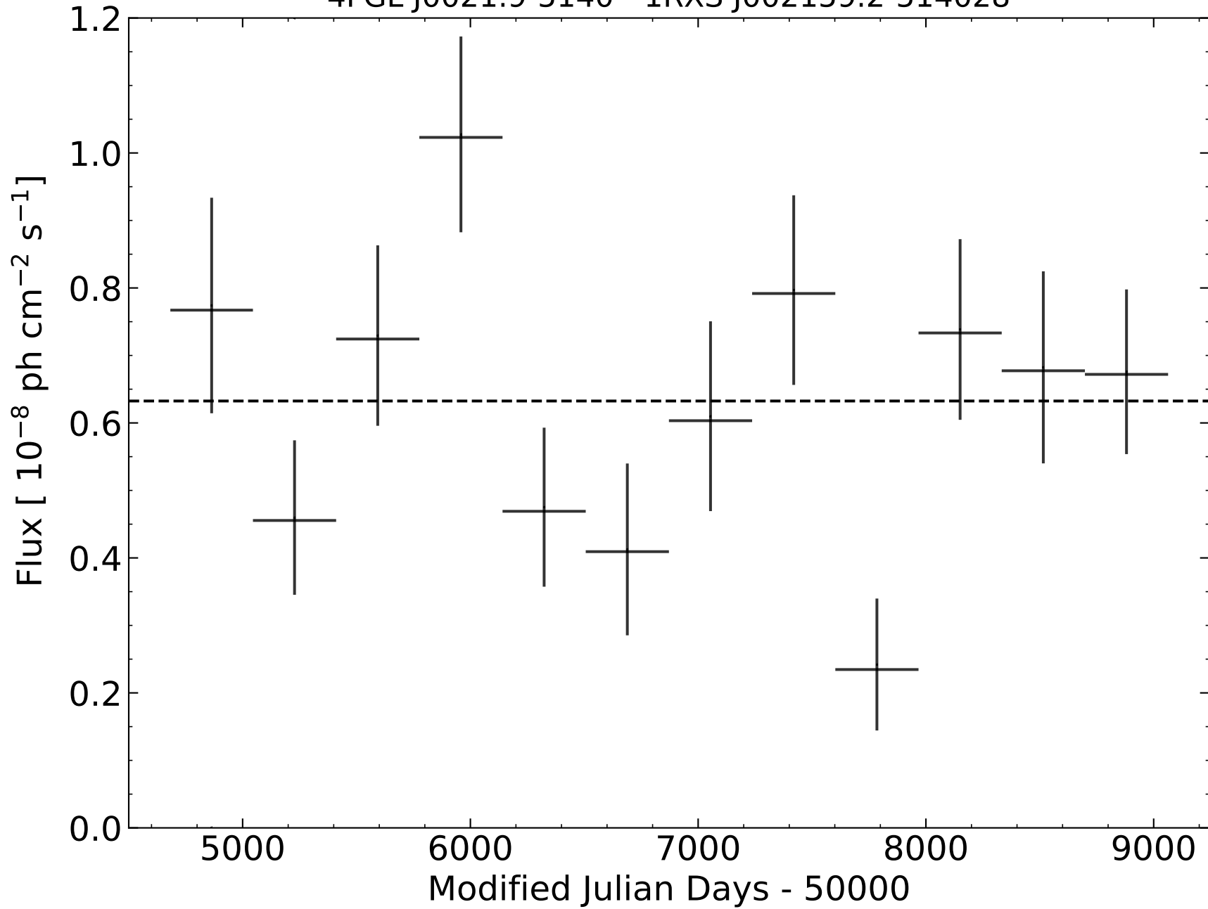
4FGL J0021.9-5140 - 1RXS J002159.2-514028
