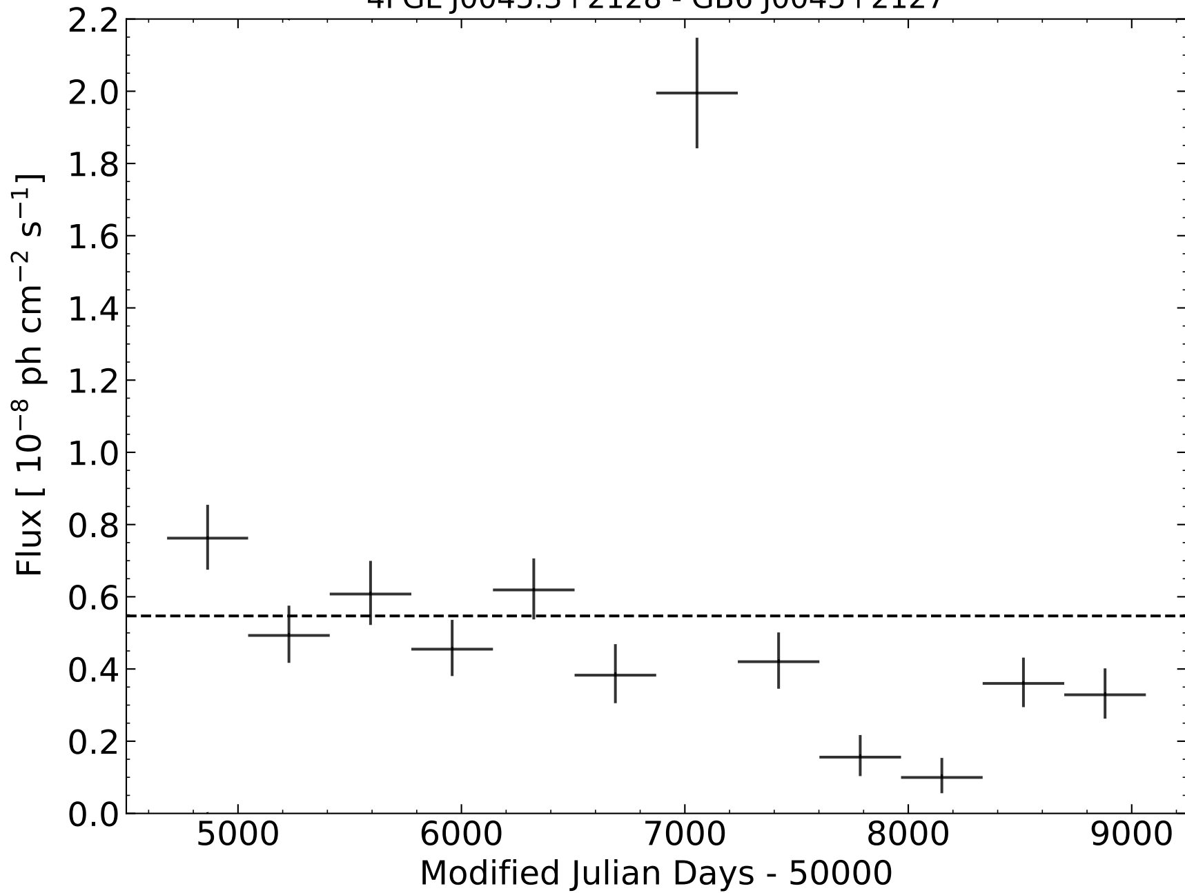
4FGL J0045.3+2128 - GB6 J0045+2127
