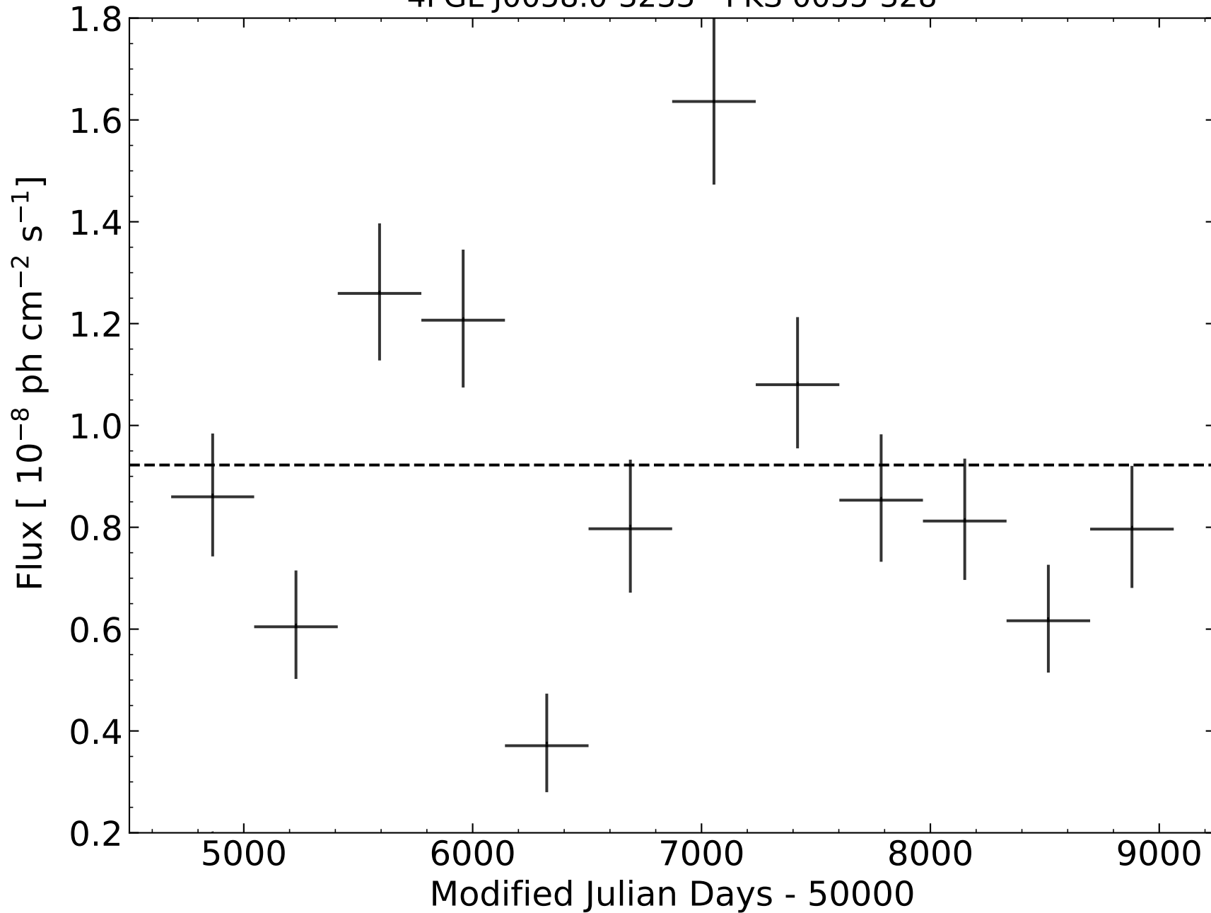
4FGL J0058.0-3233 - PKS 0055-328
