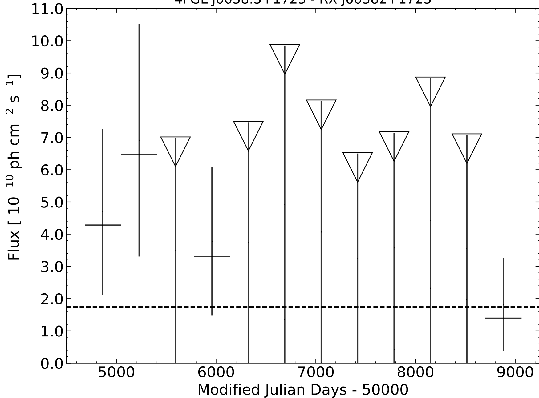
4FGL J0058.3+1723 - RX J00582+1723
