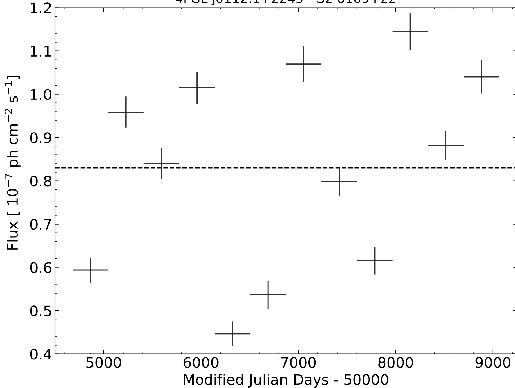
4FGL J0112.1+2245 - S2 0109+22
