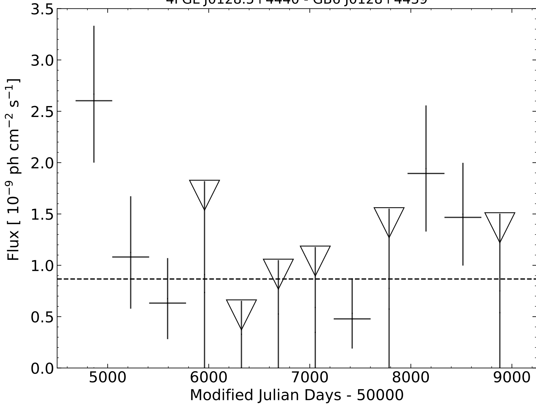
4FGL J0128.5+4440 - GB6 J0128+4439
