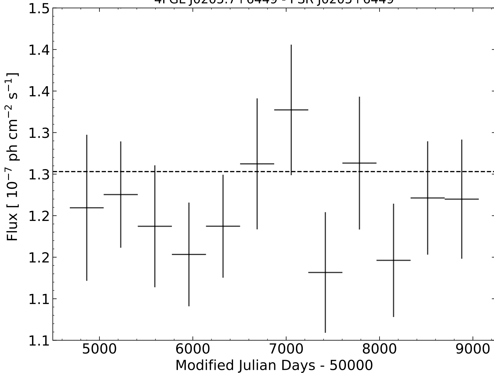
4FGL J0205.7+6449 - PSR J0205+6449
