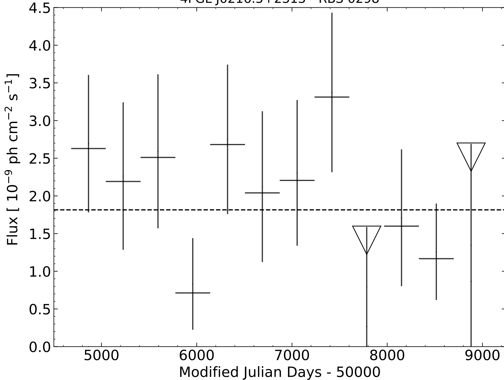
4FGL J0216.5+2313 - RBS 0298
