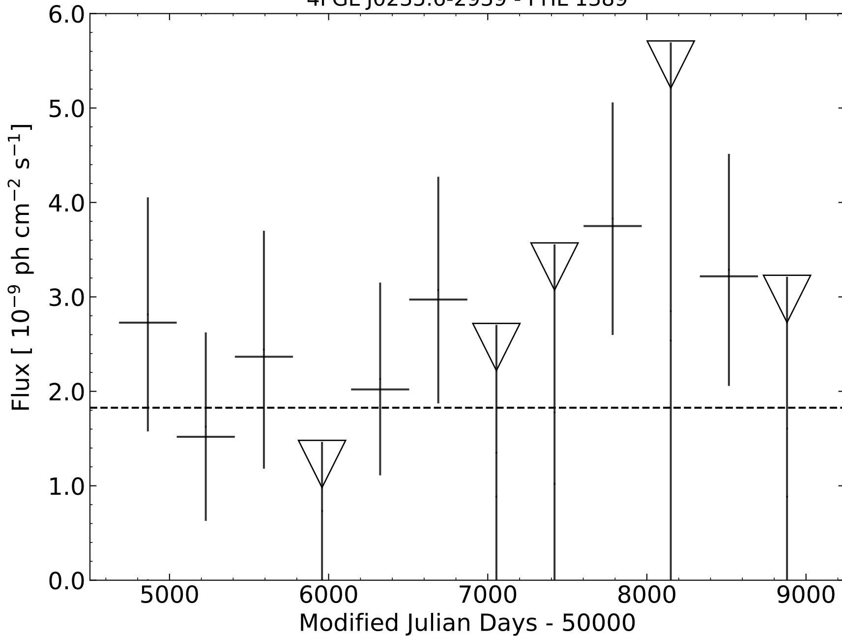
4FGL J0235.6-2939 - PHL 1389
