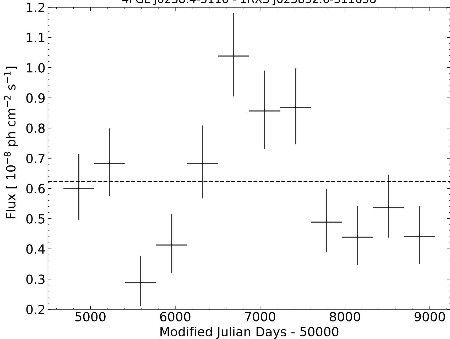
4FGL J0238.4-3116 - 1RXS J023832.6-311658
