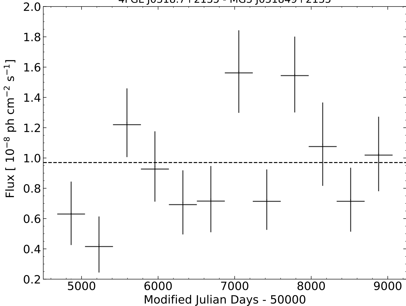
4FGL J0318.7+2135 - MG3 J031849+2135
