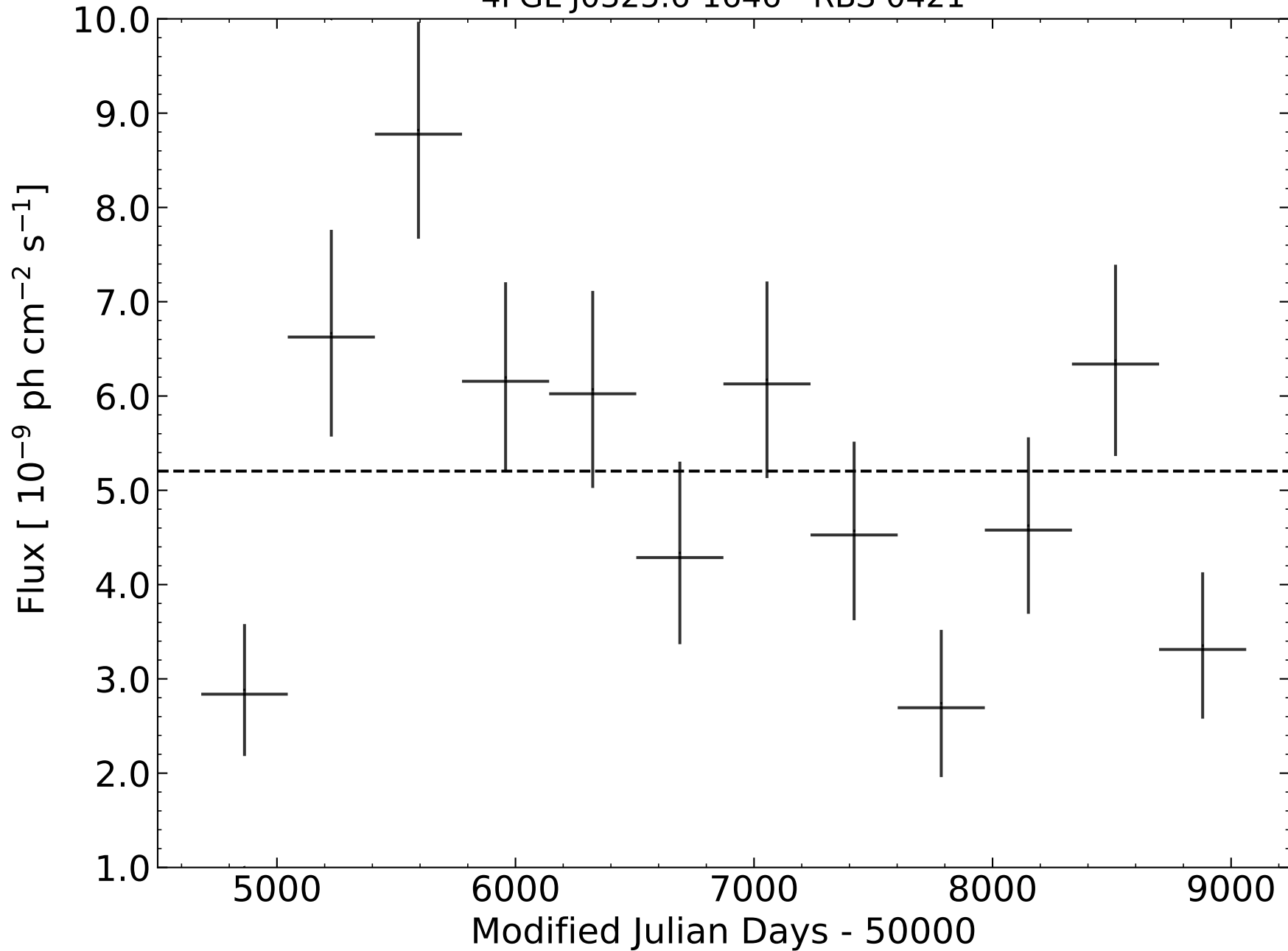
4FGL J0325.6-1646 - RBS 0421
