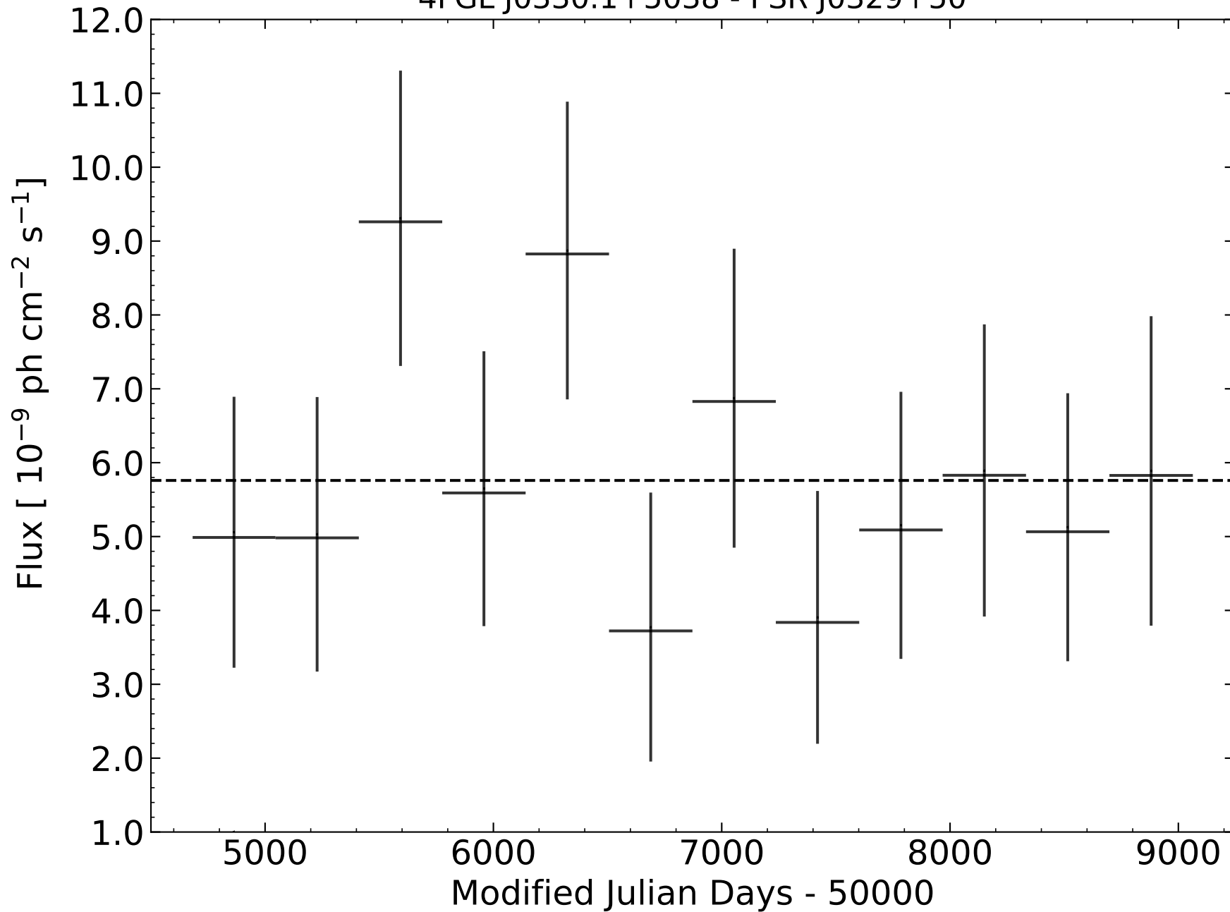
4FGL J0330.1+5038 - PSR J0329+50
