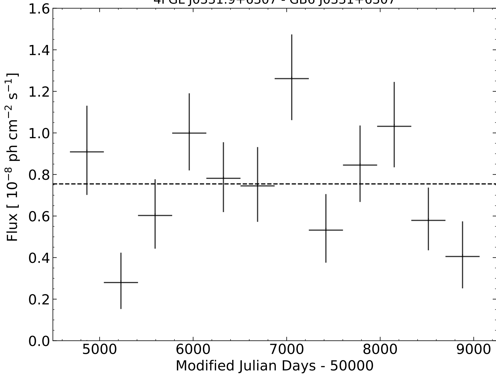
4FGL J0331.9+6307 - GB6 J0331+6307
