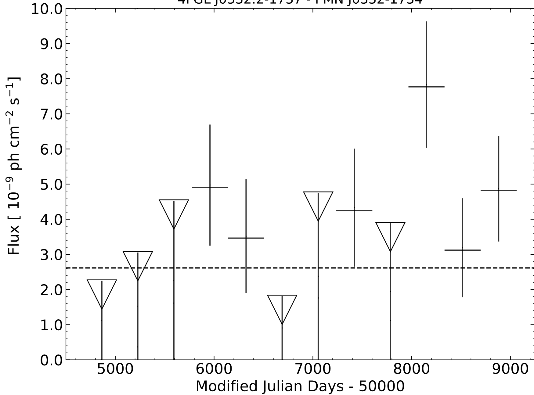
4FGL J0332.2-1737 - PMN J0332-1734
