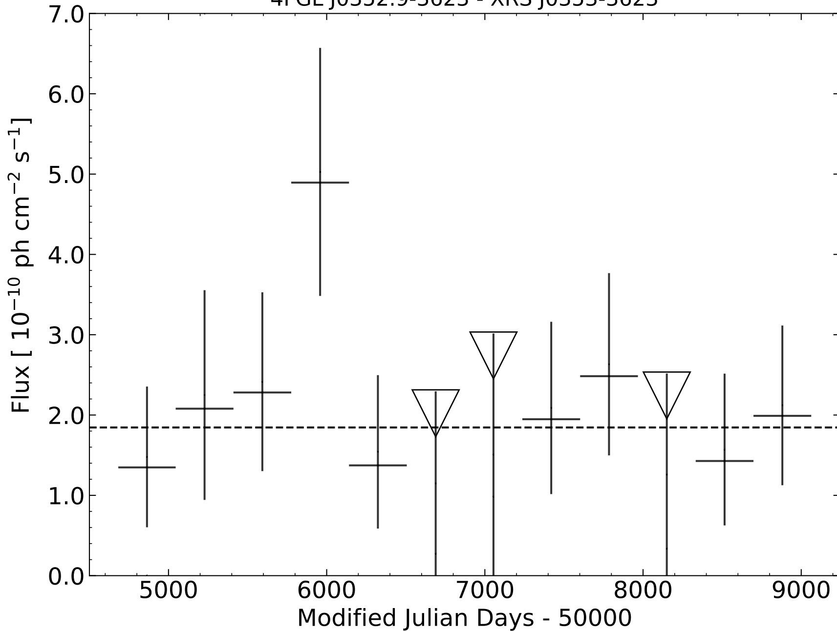
4FGL J0352.9-3623 - XRS J0353-3623
