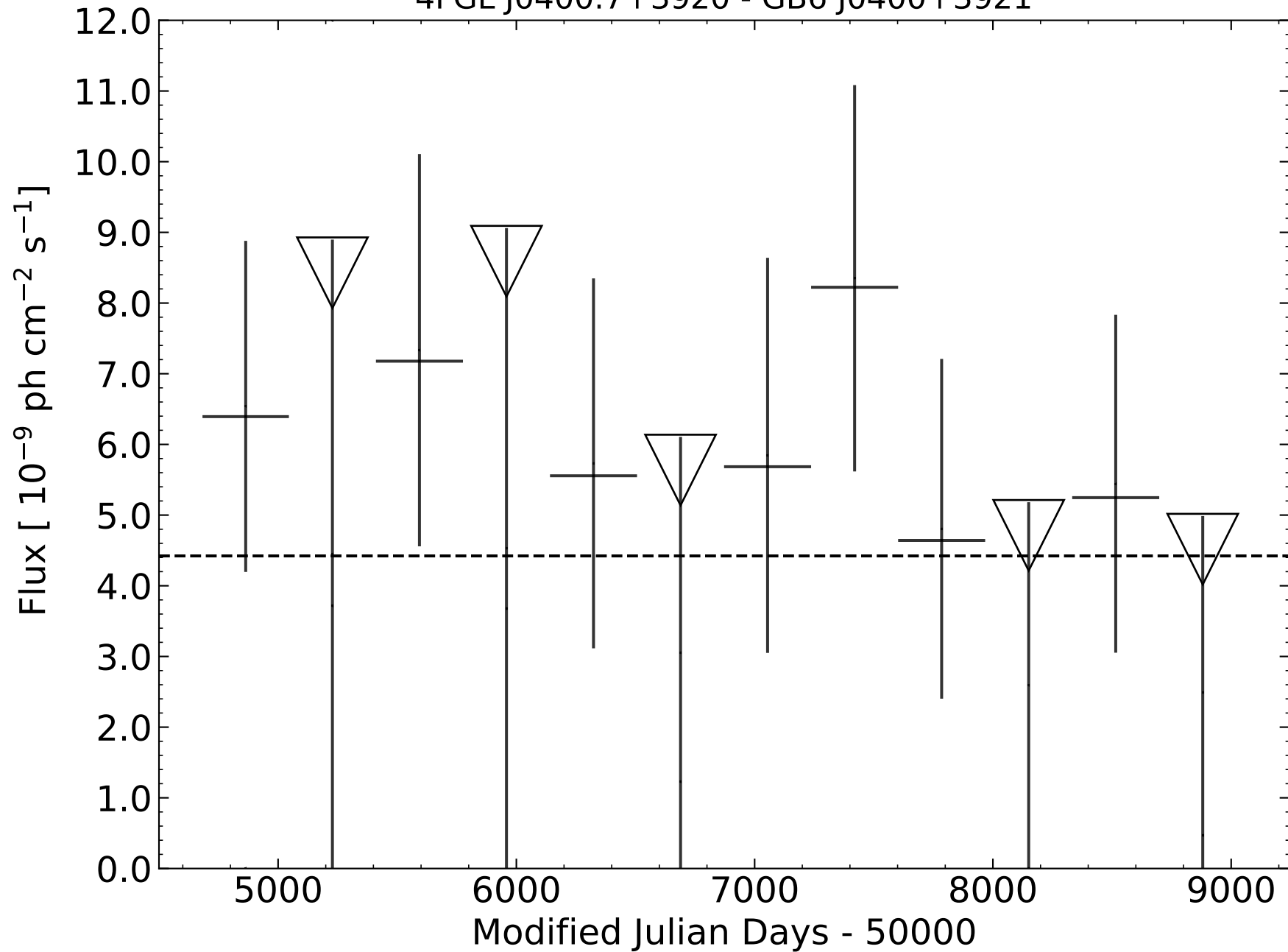
4FGL J0400.7+3920 - GB6 J0400+3921
