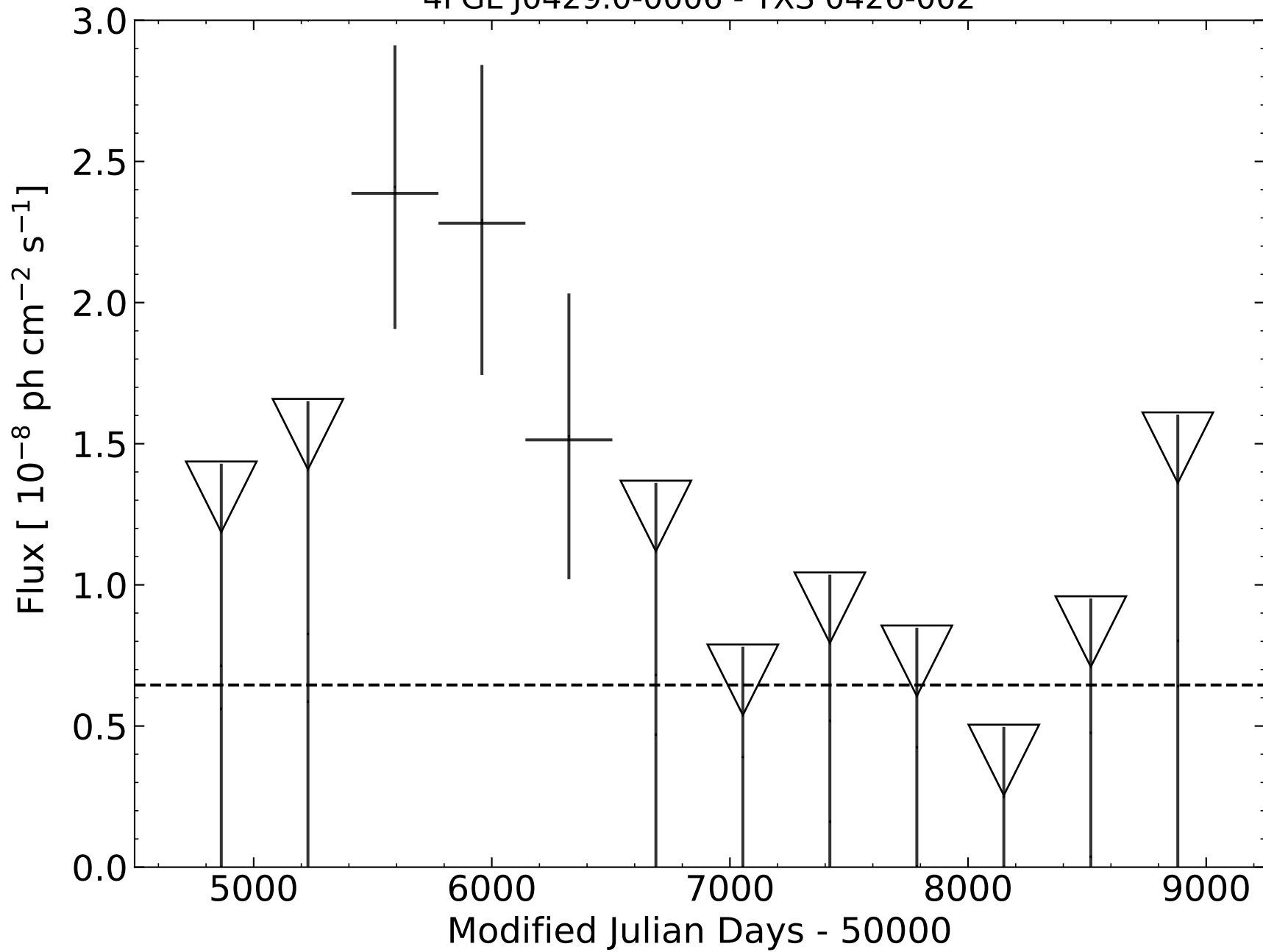
4FGL J0429.0-0006 - TXS 0426-002
