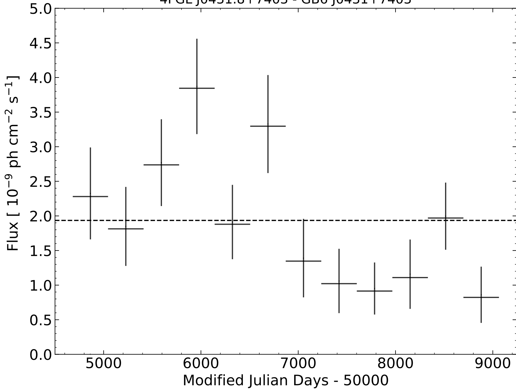
4FGL J0431.8+7403 - GB6 J0431+7403
