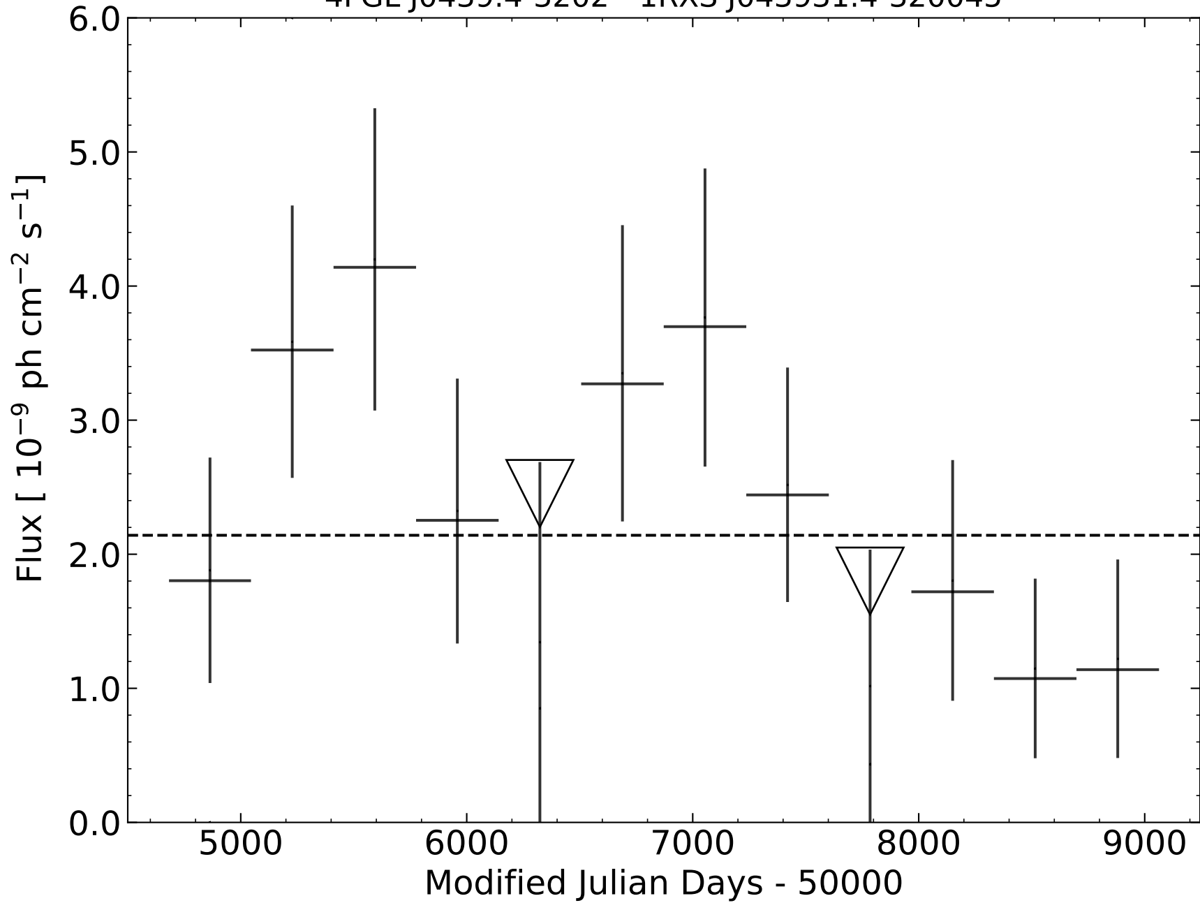
4FGL J0439.4-3202 - 1RXS J043931.4-320045
