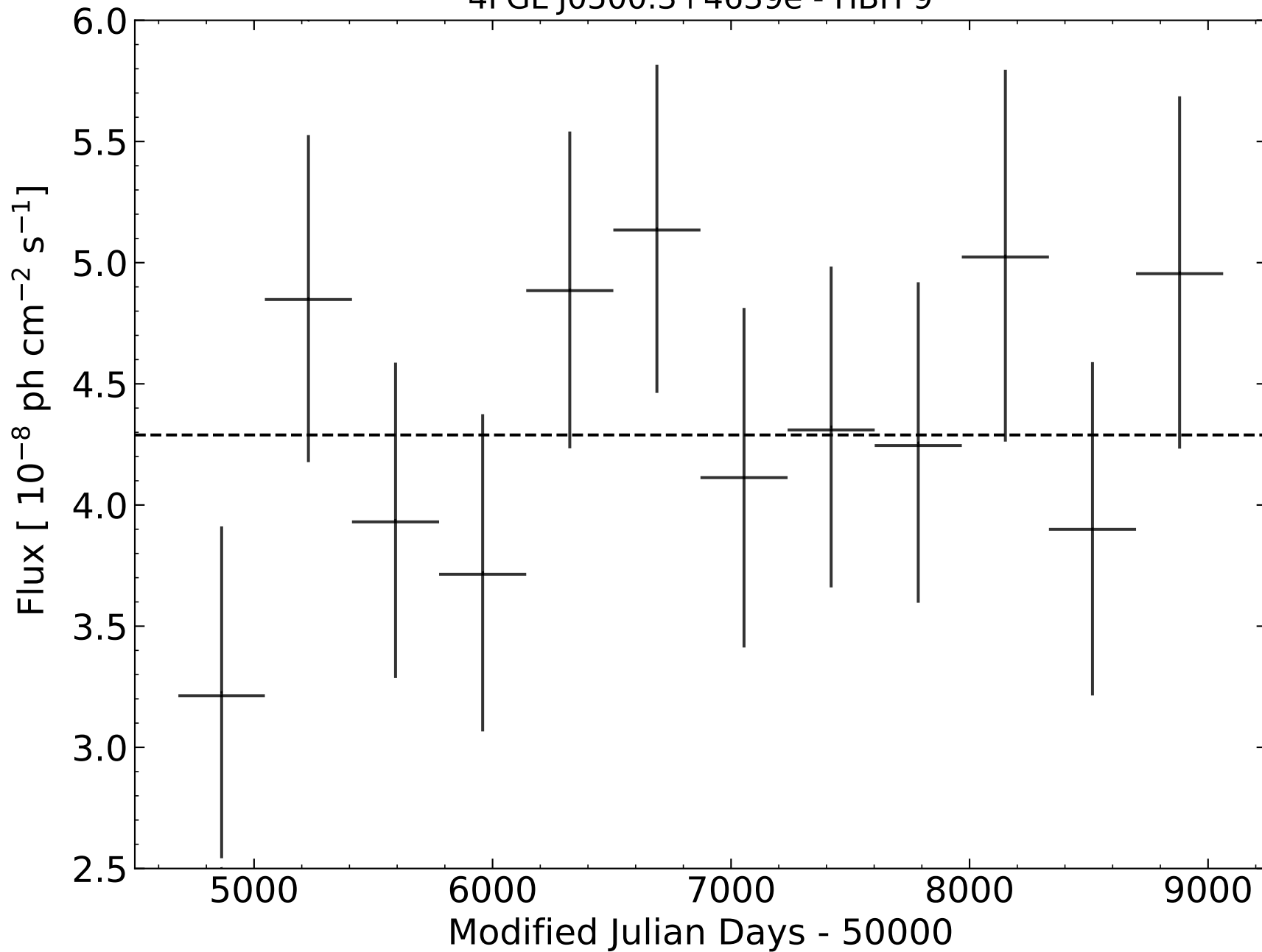
4FGL J0500.3+4639e - HBH 9
