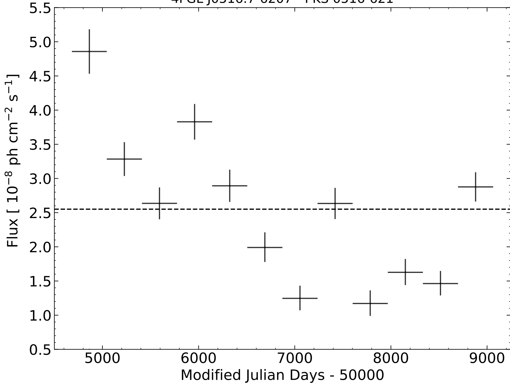
4FGL J0516.7-6207 - PKS 0516-621
