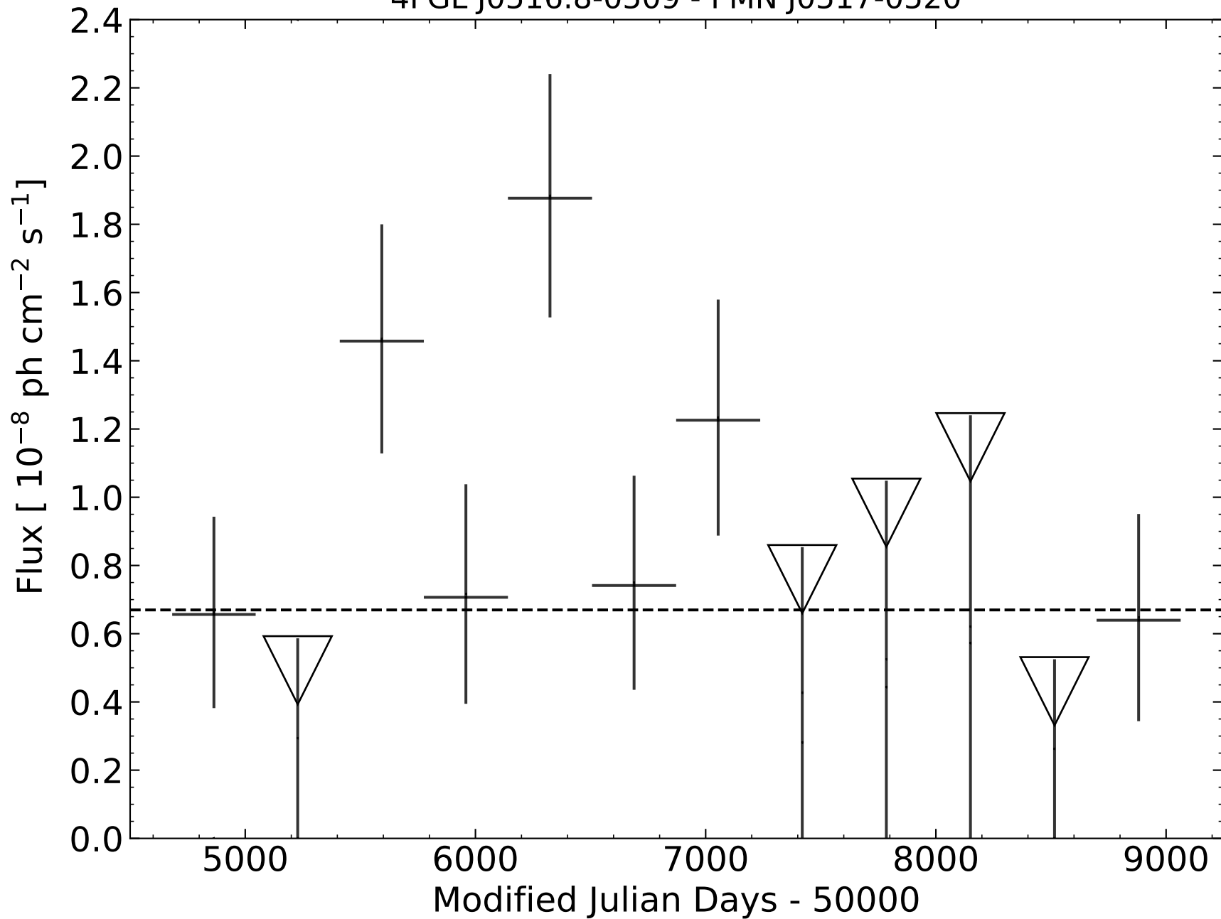
4FGL J0516.8-0509 - PMN J0517-0520
