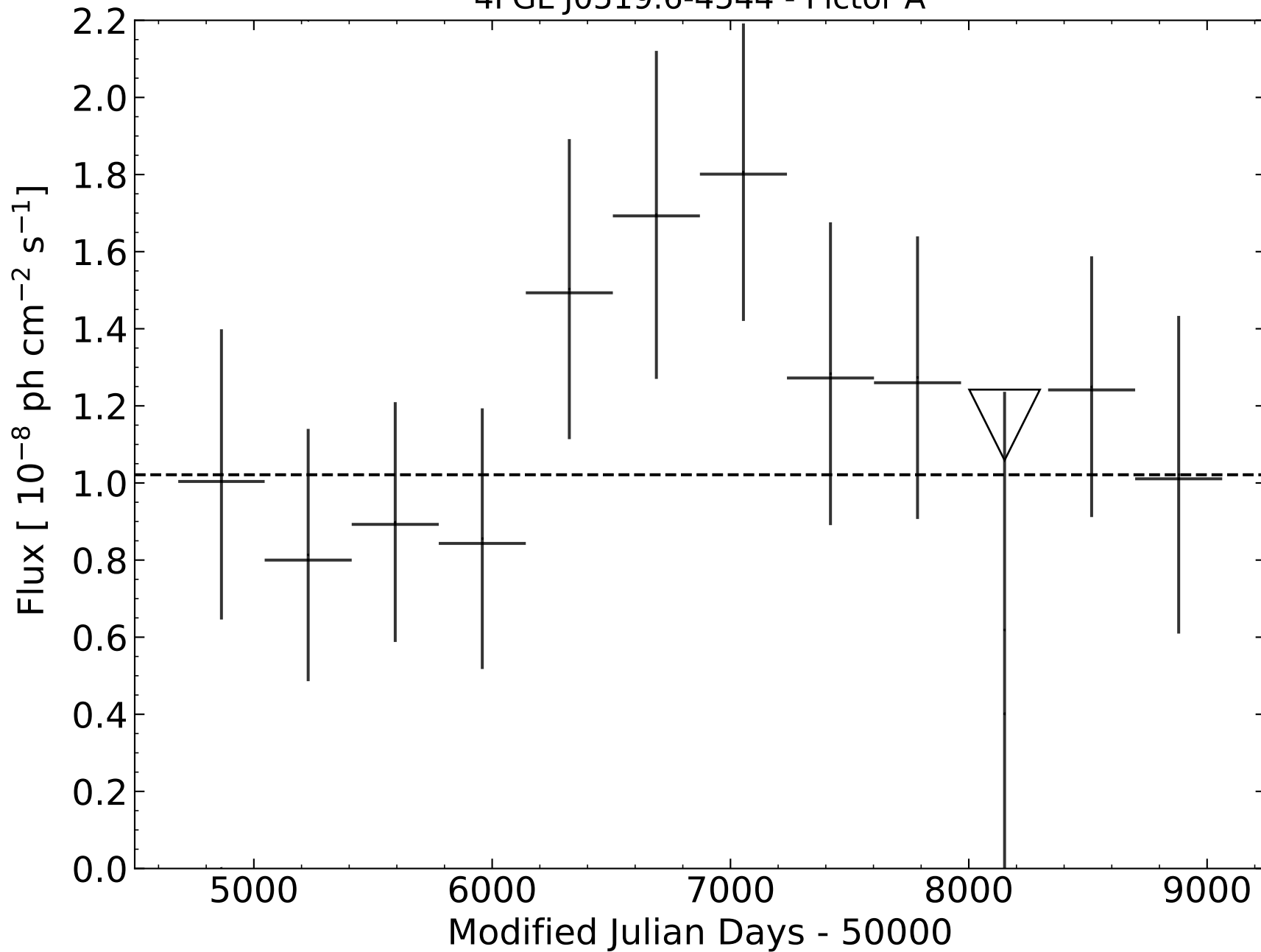
4FGL J0519.6-4544 - Pictor A
